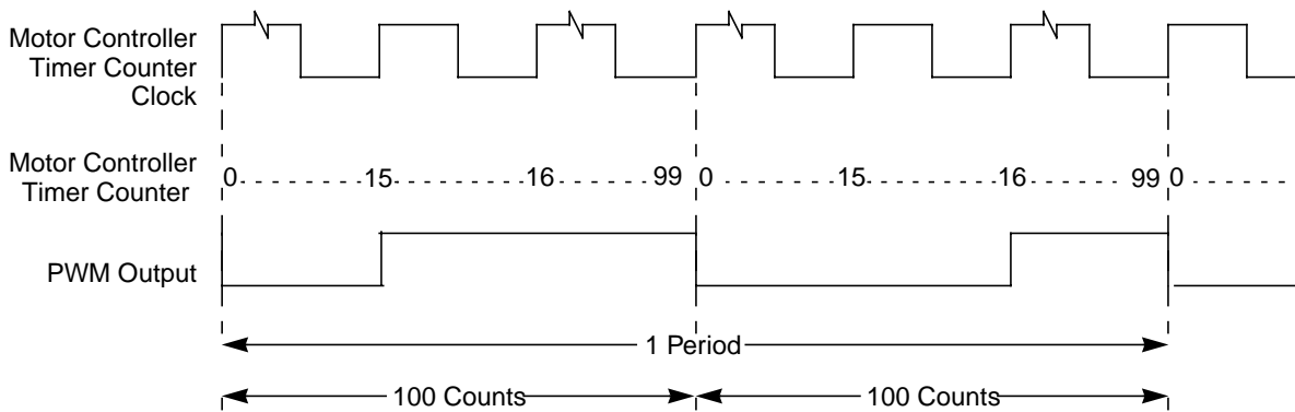
Figure 9-18. PWM Output: DITH = 1, MCAM[1:0] = 01, MCDC = 31, MCPER = 200, RECIRC = 0
