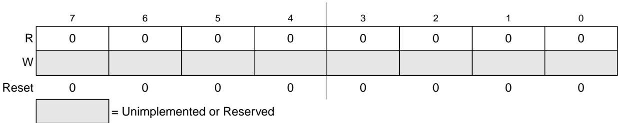
Figure 21-17. Reserved Register
