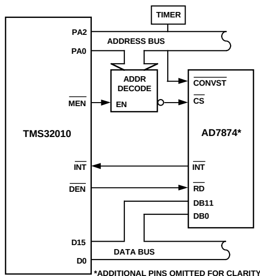
Figure 13. AD7874–TMS32010 Interface
