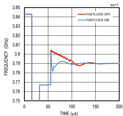
PLL LOCK vs. TIME
