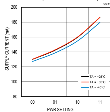
SUPPLY CURRENT vs. OUTPUT POWER SETTING (TWO CHANNELS ACTIVE, 3GHz)
