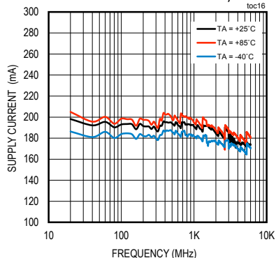
SUPPLY CURRENT vs. FREQUENCY (TWO CHANNELS ACTIVE, MAXIMUM OUTPUT POWER)
