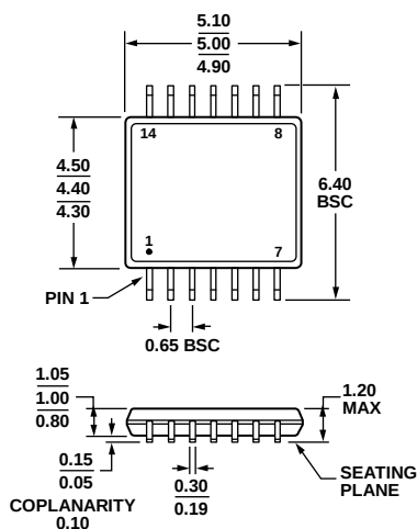
Figure 36. 14-Lead Thin Shrink Small Outline Package [TSSOP] (RU-14)
