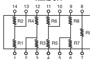
Quad Divider Feedback Network with Equal Value Resistors
