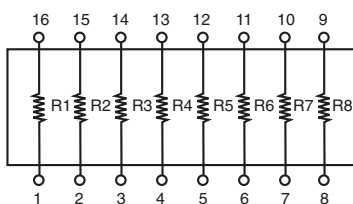
8 Equal and Independent Resistors
