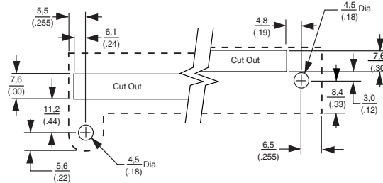
RIGHT ANGLE MOUNTING PANEL LAYOUT
