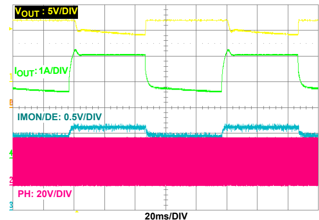
FIGURE 35. AVERAGE CONSTANT OUTPUT CURRENT CONTROL, V_{IN} = 36V , V_{OUT} \text{ (SETTING)} = 12V , C_{IMON} = 1nF , R_{IMON} = 130k\Omega , ACL = 4.05A , R_L = 5.0\Omega TO 2.0\Omega , F_{LOAD} = 10Hz , DUTY OF LOAD CHANGE = 50%
