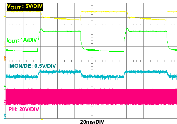
FIGURE 34. AVERAGE CONSTANT OUTPUT CURRENT CONTROL, V_{IN} = 20V , V_{OUT} \text{ (SETTING)} = 12V , C_{IMON} = 1nF , R_{IMON} = 130k\Omega , ACL = 4.05A , R_L = 5.0\Omega TO 2.0\Omega , F_{LOAD} = 10Hz , DUTY OF LOAD CHANGE = 50%
