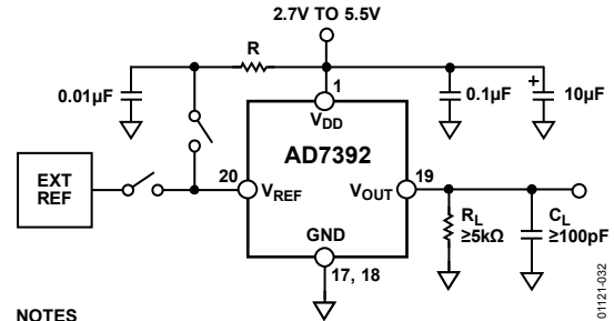
NOTES 1. DIGITAL INTERFACE CIRCUITRY OMITTED FOR CLARITY Figure 32. AD7392 Unipolar Output Operation
