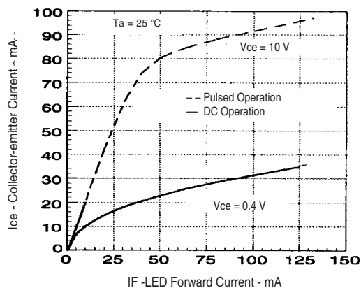
Figure 5. Non-Saturated and Saturated Collector Emitter Current vs. LED Current
