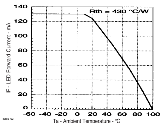
Figure 2. Maximum LED Current vs. Ambient Temperature
