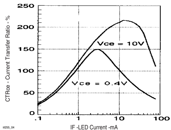
Figure 4. Current Transfer Ratio vs. LED Current and Collector-Emitter Voltage
