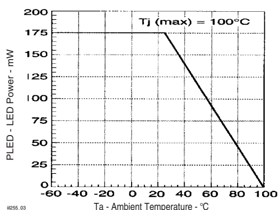
Figure 3. Maximum LED Power Dissipation
