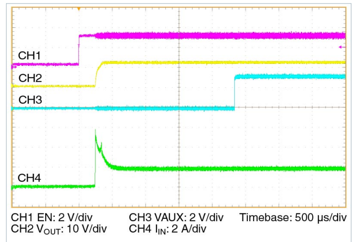
Figure 15 — Start up from application of EN with pre-applied V_{IN} = 384 V , 50% I_{OUT} , 100% C_{OUT}
