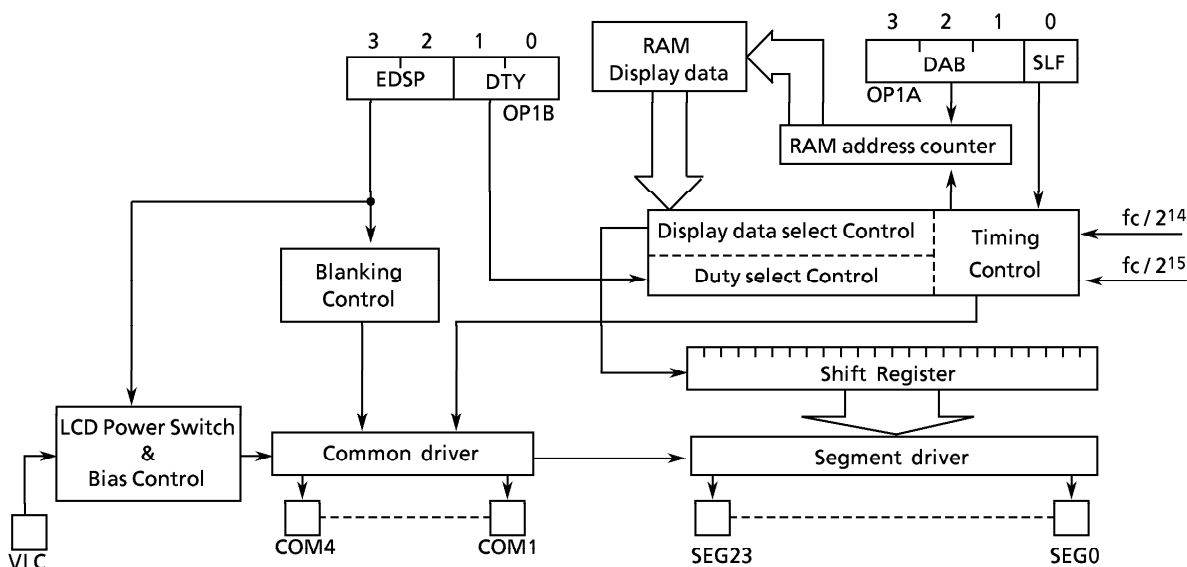
Figure 3-1. Configuration of LCD driver
