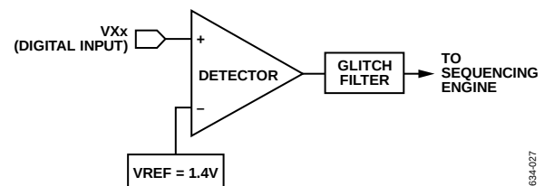
Figure 18. VXx Digital Input Function
