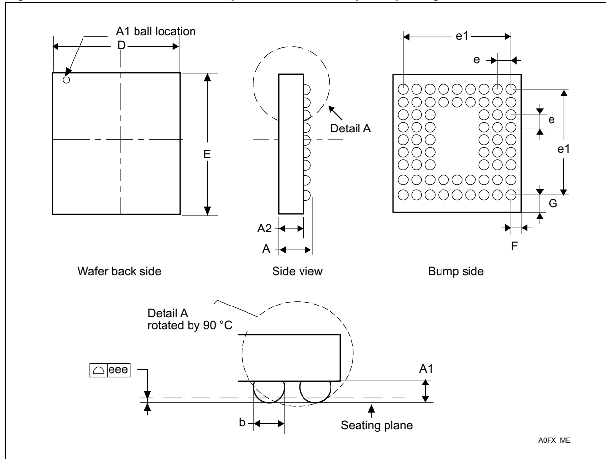
Figure 76. WLCSP64+2 - 0.400 mm pitch wafer level chip size package outline
