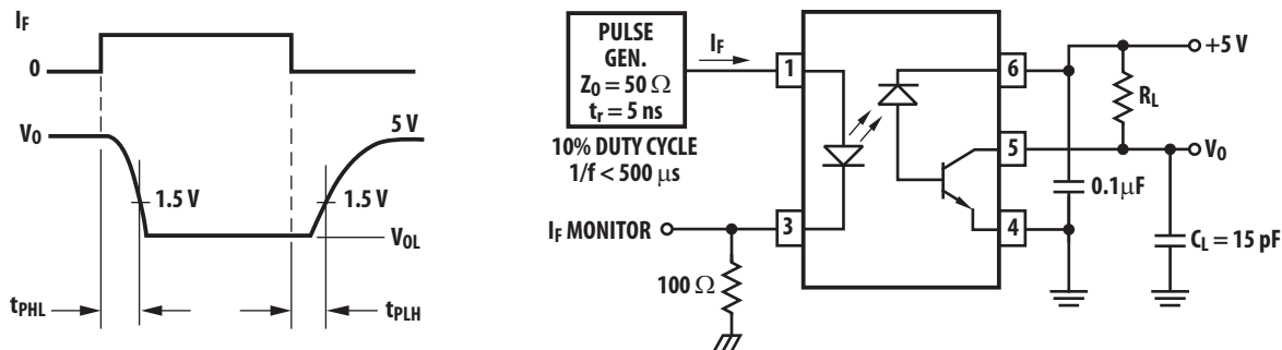
Figure 10. Switching Test Circuit.
