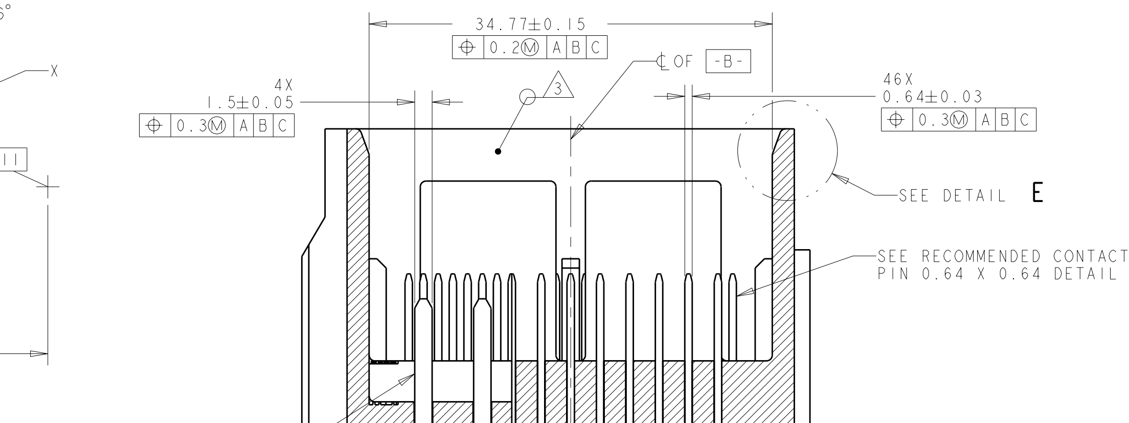
SEE RECOMMENDED CONTACT PIN 0.8 X 1.5 DETAIL
