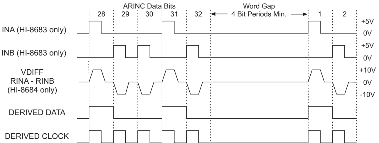
FIGURE 3 - RECEIVER INPUT TIMING FOR ARINC 429
