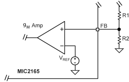
Figure 9. Voltage-Divider Configuration
