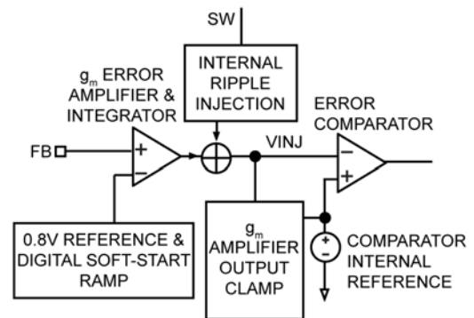
Figure 10. Internal Ripple Injection
