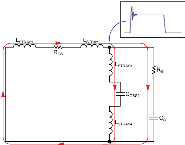
Figure 7. Snubber Circuit
