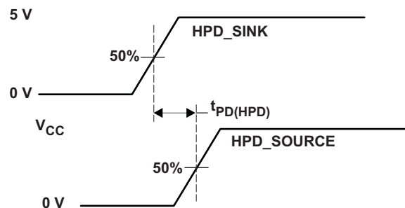
Figure 8. HPD Timing Diagram (HPDINV = LOW)
