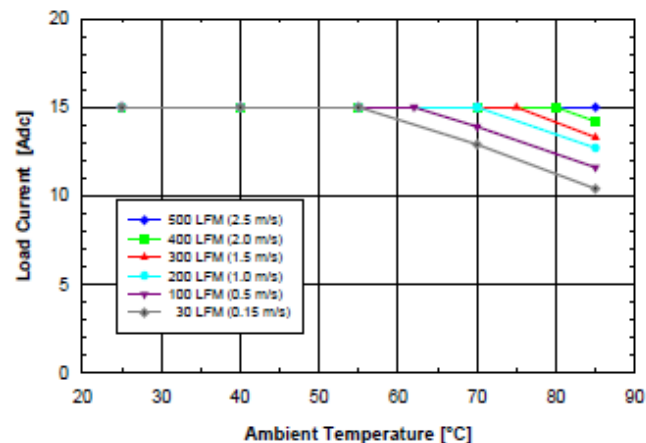
Fig. 2.5V.1: Available load current vs. ambient air temperature and airflow rates for SQ48T15025 converter with D height pins mounted vertically with Vin = 48 V, air flowing from pin 3 to pin 1, and maximum FET temperature ≤ 120 °C.
