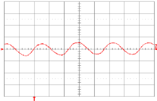
Fig. 6.0V.15: Input reflected ripple current, i_c (100 mA/div.), measured at input terminals at full rated load current and V_{in} = 48\text{V} . Refer to Fig. 6.0V.14 for test setup. Time scale: 1\ \mu\text{s}/\text{div} .
