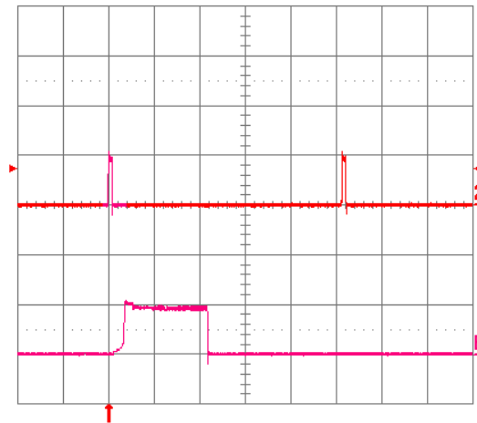
Fig. 3.3V.18: Load current (top trace, 20 A/div., 20 ms/div.) into a 10 mΩ short circuit during restart, at V_{in} = 48 V. Bottom trace (20 A/div., 1 ms/div.) is an expansion of the on-time portion of the top trace.
