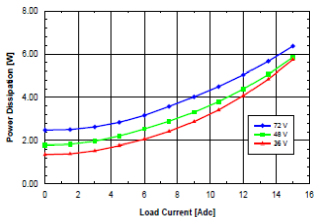
Fig. 3.3V.7: Power dissipation vs. load current and input voltage for SQ48T/S15033 converter mounted vertically with air flowing from pin 3 to pin 1 at a rate of 300 LFM (1.5 m/s) and T_a = 25^\circ\text{C} .
