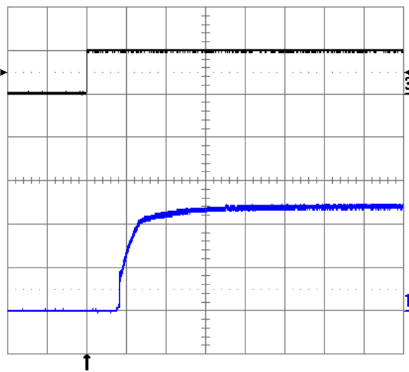
Fig. 1.2V.10: Turn-on transient at full rated load current (resistive) plus 10,000 \mu\text{F} at V_{in} = 48\text{ V} , triggered via ON/OFF pin. Top trace: ON/OFF signal (5 V/div.). Bottom trace: output voltage (0.5 V/div.). Time scale: 2 ms/div.
