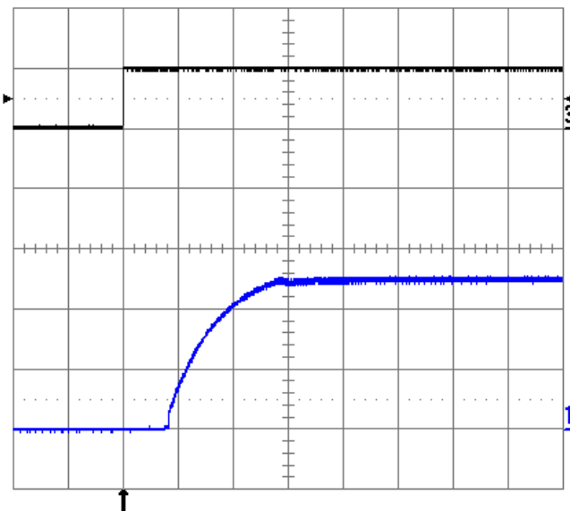
Fig. 2.5V.10: Turn-on transient at full rated load current (resistive) plus 10,000 \mu\text{F} at V_{in} = 48\text{V} , triggered via ON/OFF pin. Top trace: ON/OFF signal (5 V/div.). Bottom trace: output voltage (1 V/div.). Time scale: 2 ms/div.
