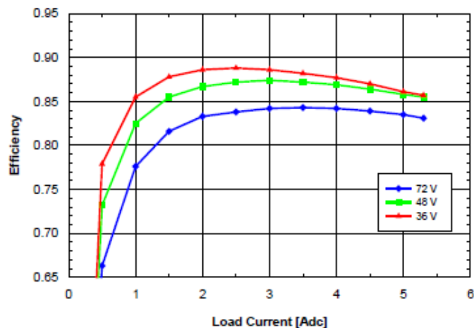
Fig. 8.0V.5: Efficiency vs. load current and input voltage or SQ48T/S05080 converter mounted vertically with air flowing from pin 3 to pin 1 at a rate of 300 LFM (1.5 m/s) and T_a = 25^{\circ}C .
