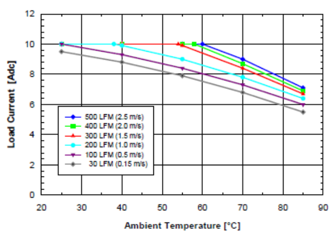
Fig. 5.0V.4: Available load current vs. ambient air temperature and airflow rates for SQ48S10050 converter mounted horizontally with Vin = 48V, air flowing from pin 3 to pin 1, and maximum FET temperature ≤ 120°C.
