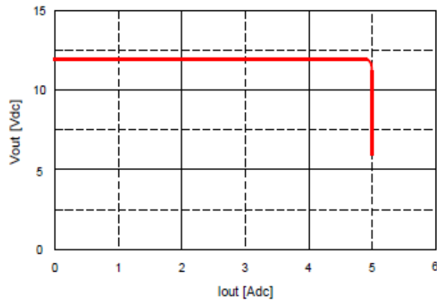
Fig. 12V.17: Output voltage vs. load current showing current limit point and converter shutdown point. Input voltage has almost no effect on current limit characteristic.
