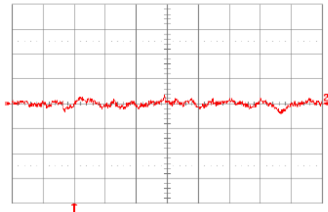
Fig. 5.0V.16: Input reflected ripple current, i_s (10 mA/div.), measured through 10\ \mu\text{H} at the source at full rated load current and V_{in} = 48\text{V} . Refer to Fig. 5.0V.14 for test setup. Time scale: 1\ \mu\text{s}/\text{div} .
