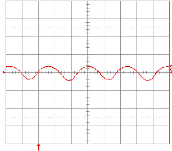
Fig. 1.8V.15: Input reflected ripple current, i_c (100 mA/div.), measured at input terminals at full rated load current and V_{in} = 48 V. Refer to Fig. 1.8V.14 for test setup. Time scale: 1 \mu s/div.
