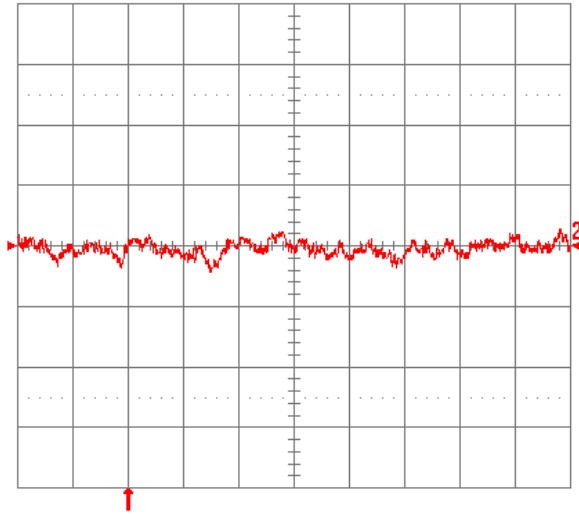
Fig. 1.8V.16: Input reflected ripple current, i_s (10 mA/div.), measured through 10 \mu H at the source at full rated load current and V_{in} = 48 V. Refer to Fig. 1.8V.14 for test setup. Time scale: 1 \mu s/div.
