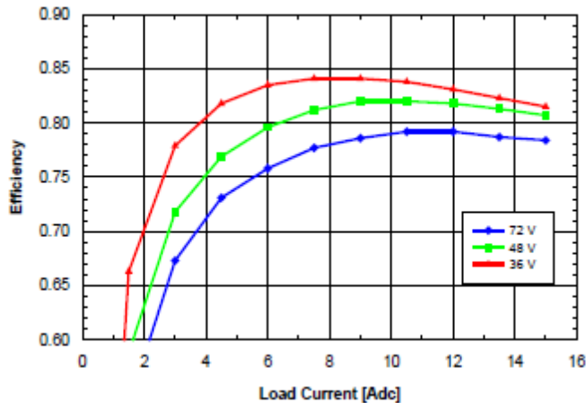
Fig. 1.0V.5: Efficiency vs. load current and input voltage for SQ48T/S15010 converter mounted vertically with air flowing from pin 3 to pin 1 at a rate of 300 LFM (1.5 m/s) and T_a = 25\text{ }^{\circ}\text{C} .
