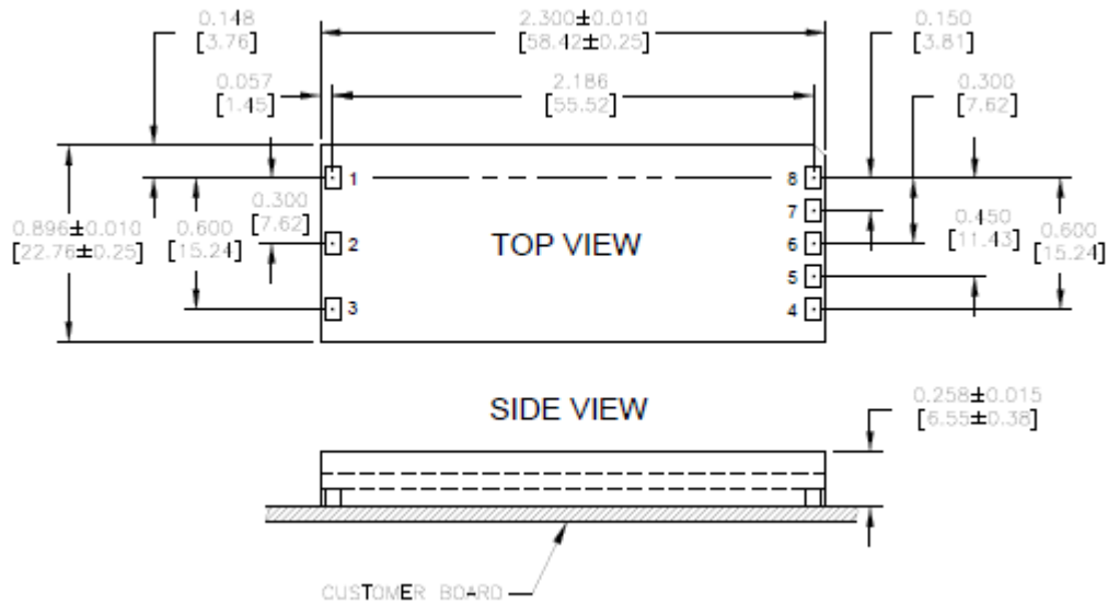
SQ48S Pinout (Surface Mount)
