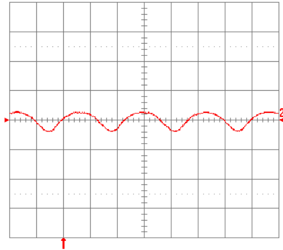
Fig. 1.2V.15: Input reflected ripple current, i_c (100 mA/div.), measured at input terminals at full rated load current and V_{in} = 48 V. Refer to Fig. 1.2V.14 for test setup. Time scale: 1 \mu s/div.
