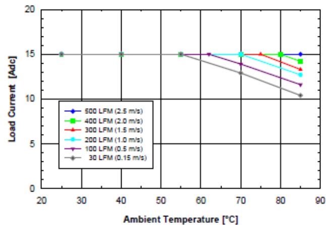
Fig. 2.5V.1: Available load current vs. ambient air temperature and airflow rates for SQ48T15025 converter with D height pins mounted vertically with Vin = 48 V, air flowing from pin 3 to pin 1, and maximum FET temperature ≤ 120 °C.
