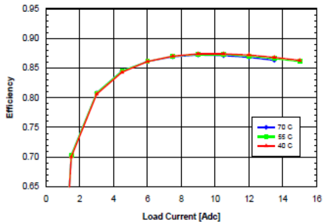
Fig. 2.0V.6: Efficiency vs. load current and ambient for SQ48T/S15020 converter mounted vertically with air flowing from pin 3 to pin 1 at a rate of 200 LFM (1.0 m/s).
