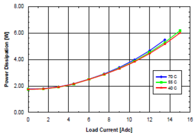
Fig. 3.3V.8: Power dissipation vs. load current and ambient temperature for SQ48T/S15033 converter mounted vertically with V_{in} = 48\text{V} and air flowing from pin 3 to pin 1 at a rate of 200 LFM (1.0 m/s).
