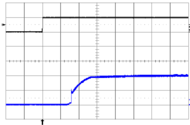
Fig. 1.0V.10: Turn-on transient at full rated load current (resistive) plus 10,000 \mu\text{F} at V_{in} = 48\text{ V} , triggered via ON/OFF pin. Top trace: ON/OFF signal (5 V/div.). Bottom trace: output voltage (0.5 V/div.). Time scale: 2 ms/div.
