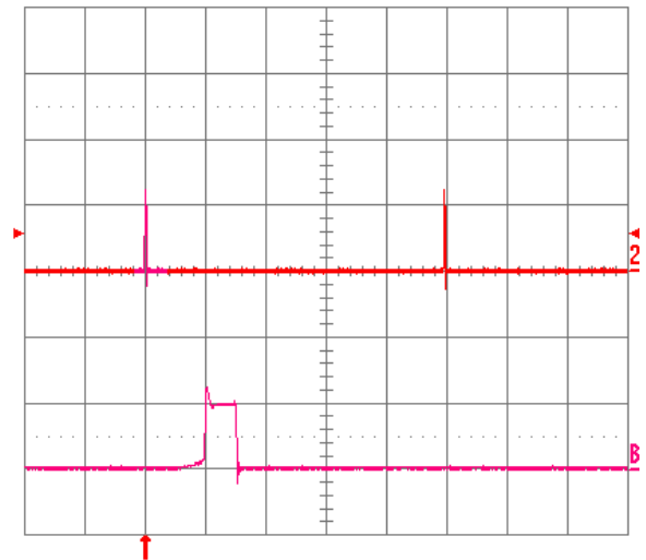
Fig. 2.5V.18: Load current (top trace, 20 A/div., 20 ms/div.) into a 10 m \Omega short circuit during restart, at V_{in} = 48 V. Bottom trace (20 A/div., 1 ms/div.) is an expansion of the on-time portion of the top trace.
