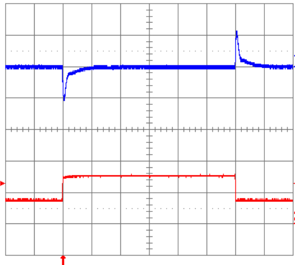
Fig. 1.5V.12: Output voltage response to load current step-change (3.75 A – 7.5 A – 3.75 A) at V_{in} = 48 V. Top trace: output voltage (100 mV/div.). Bottom trace: load current (5 A/div.). Current slew rate: 5 A/ \mu s. C_o = 450 \mu F tantalum + 1 \mu F ceramic. Time scale: 0.2 ms/div.
