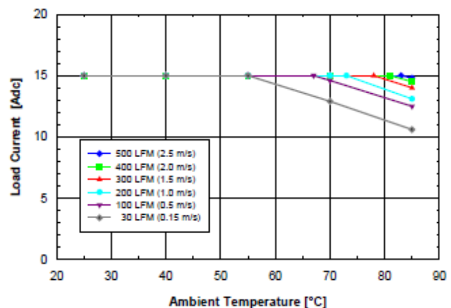
Fig. 2.5V.4: Available load current vs. ambient air temperature and airflow rates for SQ48S15025 converter
