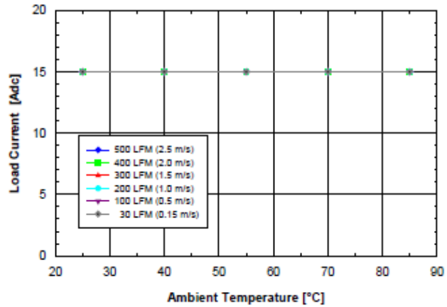
Fig. 1.0V.4: Available load current vs. ambient air temperature and airflow rates for SQ48S15010 converter mounted horizontally with V_{in} = 48\text{ V} , air flowing from pin 3 to pin 1, and maximum FET temperature \leq 120\text{ }^{\circ}\text{C} .
