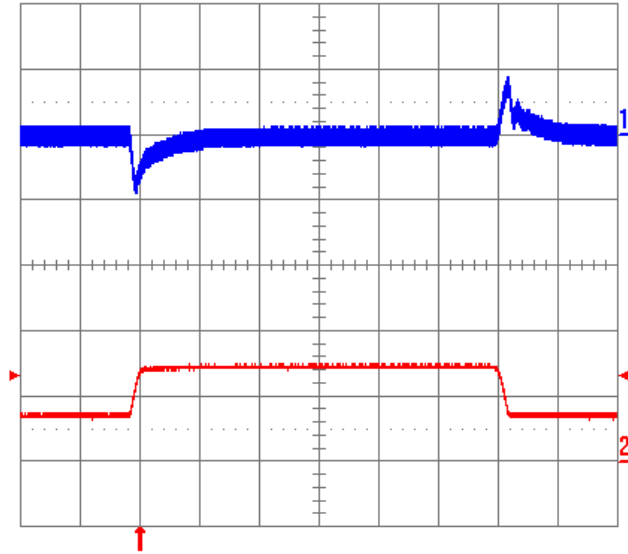
Fig. 1.8V.11: Output voltage response to load current step-change (3.75 A – 7.5 A – 3.75 A) at V_{in} = 48 V. Top trace: output voltage (100 mV/div.). Bottom trace: load current (5 A/div.). Current slew rate: 0.1 A/ \mu s. C_o = 1 \mu F ceramic. Time scale: 0.2 ms/div.
