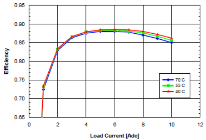
Fig. 5.0V.6: Efficiency vs. load current and ambient temperature for SQ48T/S10050 converter mounted vertically with V_{in} = 48\text{V} and air flowing from pin 3 to pin 1 at a rate of 200 LFM (1.0m/s).
