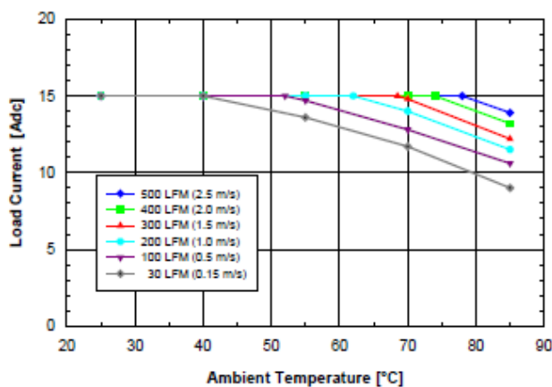
Fig. 3.3V.1: Available load current vs. ambient air temperature and airflow rates for SQ48T15033 converter with D height pins mounted vertically with Vin = 48V, air flowing from pin 3 to pin 1, and maximum FET temperature ≤ 120°C.
