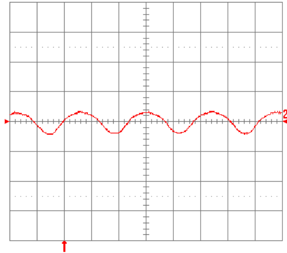
Fig. 1.5V.15: Input reflected ripple current, i_c (100 mA/div.), measured at input terminals at full rated load current and V_{in} = 48 V. Refer to Fig. 1.5V.14 for test setup. Time scale: 1 \mu s/div.
