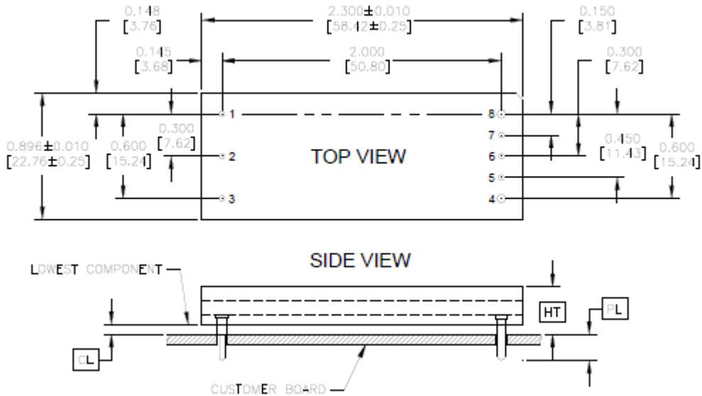
SQ48T Pinout (Through-hole)
