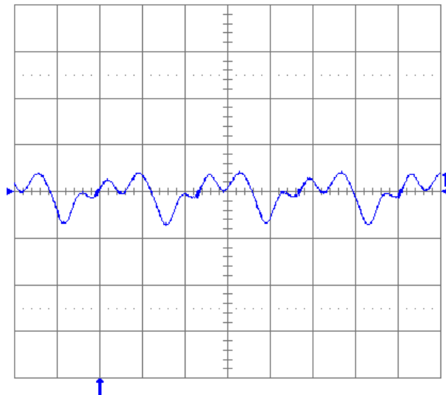
Fig. 2.0V.13: Output voltage ripple (20 mV/div.) at full rated load current into a resistive load with C_o = 10 \mu F tantalum + 1 \mu F ceramic and V_{in} = 48 V. Time scale: 1 \mu s/div.
