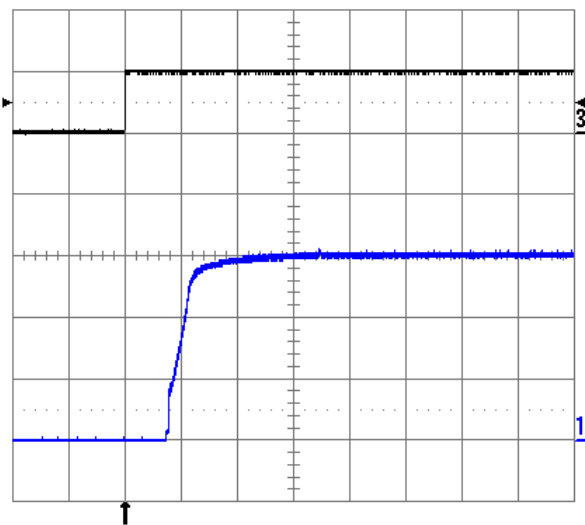
Fig. 1.5V.9: Turn-on transient at full rated load current (resistive) with no output capacitor at V_{in} = 48\text{ V} , triggered via ON/OFF pin. Top trace: ON/OFF signal (5 V/div.). Bottom trace: output voltage (0.5 V/div.). Time scale: 2 ms/div.
