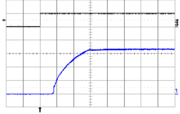
Fig. 3.3V.10: Turn-on transient at full rated load current (resistive) plus 10,000 \mu F at V_{in} = 48 V, triggered via ON/OFF pin. Top trace: ON/OFF signal (5 V/div.). Bottom trace: output voltage (1 V/div.). Time scale: 2 ms/div.
