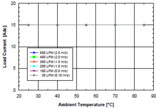
Fig. 1.0V.3: Available load current vs. ambient air temperature and airflow rates for SQ48S15010 converter mounted vertically with V_{in} = 48\text{ V} , air flowing from pin 3 to pin 1, and maximum FET temperature \leq 120\text{ }^{\circ}\text{C} .
