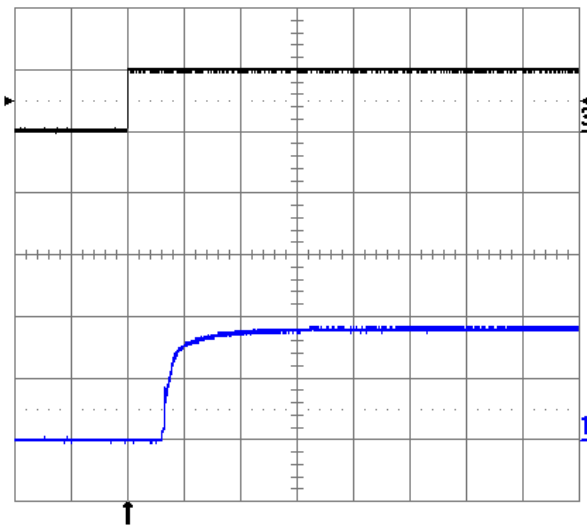
Fig. 1.8V.9: Turn-on transient at full rated load current (resistive) with no output capacitor at V_{in} = 48\text{ V} , triggered via ON/OFF pin. Top trace: ON/OFF signal (5 V/div.). Bottom trace: output voltage (1 V/div.). Time scale: 2 ms/div.
