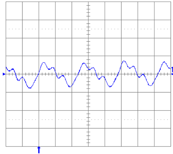
Fig. 3.3V.13: Output voltage ripple (20 mV/div.) at full rated load current into a resistive load with C_o = 10\ \mu\text{F} tantalum + 1\ \mu\text{F} ceramic and V_{in} = 48\ \text{V} . Time scale: 1\ \mu\text{s}/\text{div} .
