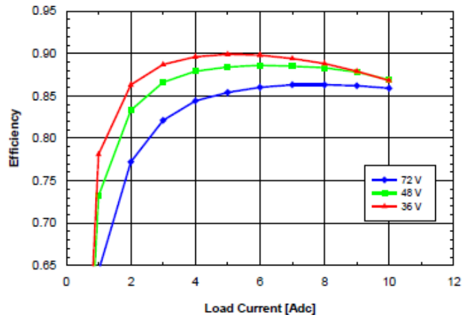
Fig. 5.0V.5: Efficiency vs. load current and input voltage for SQ48T/S10050 converter mounted vertically with air flowing from pin 3 to pin 1 at a rate of 300 LFM (1.5 m/s) and T_a = 25^\circ\text{C} .
