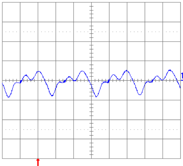
Fig. 1.8V.13: Output voltage ripple (20 mV/div.) at full rated load current into a resistive load with C_o = 10 \mu F tantalum + 1 \mu F ceramic and V_{in} = 48 V. Time scale: 1 \mu s/div.
