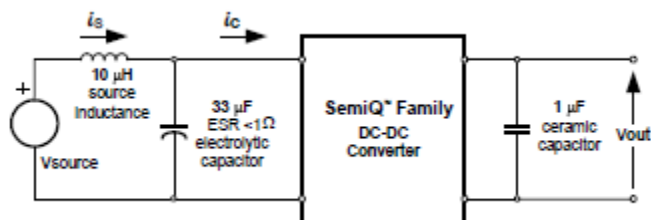
Fig. 1.0V.14: Test Setup for measuring input reflected ripple currents, i_c and i_s
