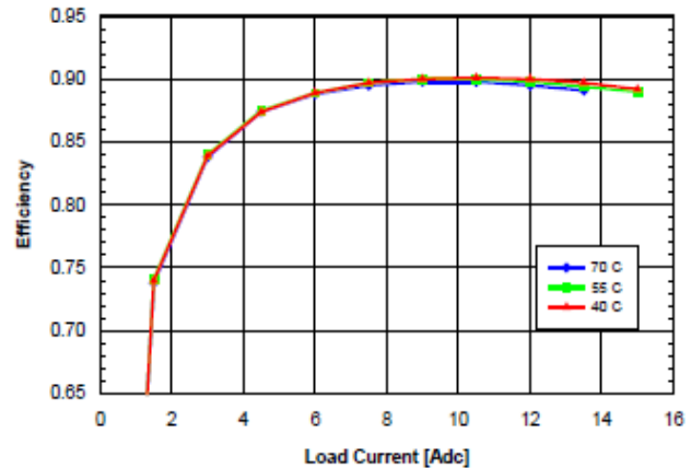
Fig. 3.3V.6: Efficiency vs. load current and ambient temperature for SQ48T/S15033 converter mounted vertically with V_{in} = 48\text{V} and air flowing from pin 3 to pin 1 at a rate of 200 LFM (1.0m/s).
