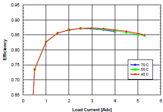
Fig. 8.0V.6: Efficiency vs. load current and ambient temperature for SQ48T/S05080 converter mounted vertically with V_{in} = 4V and air flowing from pin 3 to pin 1 at a rate of 200 LFM (1.0 m/s).
