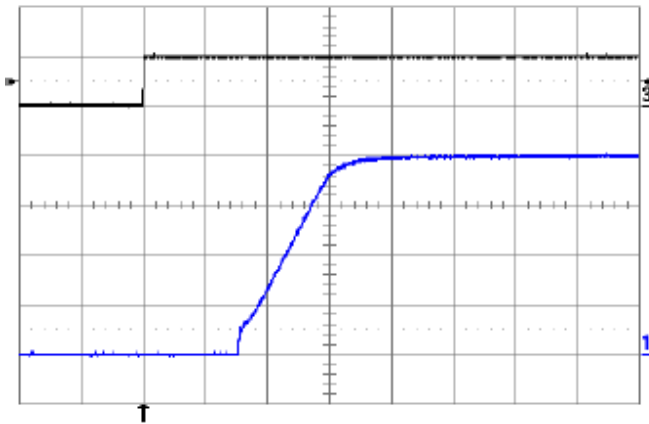
Fig. 8.0V.9: Turn-on transient at full rated load current (resistive) with no output capacitor at V_{in} = 48\text{V} , triggered via ON/OFF pin. Top trace: ON/OFF signal (5 V/div.). Bottom trace: output voltage (2 V/div.). Time scale: 1 ms/div.
