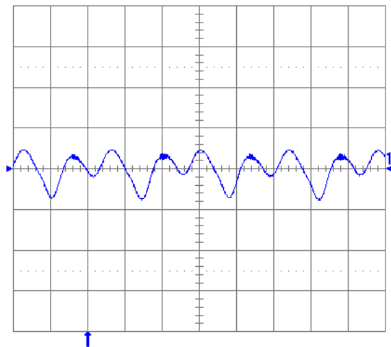
Fig. 1.5V.13: Output voltage ripple (20 mV/div.) at full rated load current into a resistive load with C_o = 10 \mu F tantalum + 1 \mu F ceramic and V_{in} = 48 V. Time scale: 1 \mu s/div.
