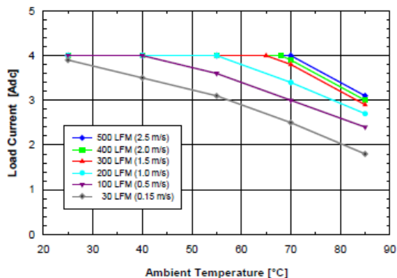
Fig. 12V.2: Available load current vs. ambient air temperature and airflow rates for SQ48T04120 converter with D height pins mounted horizontally with V_{in} = 48\text{V} , air flowing from pin 3 to pin 1, and maximum FET temperature \leq 120^\circ\text{C} .
