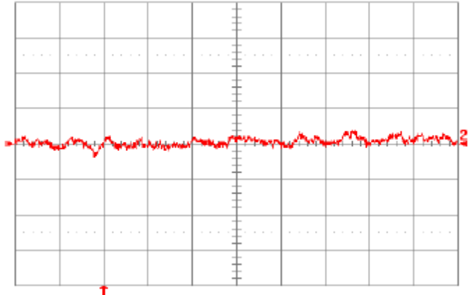
Fig. 12V.16: Input reflected ripple current, i_s (100 mA/div.), measured at input terminals at full rated load current and V_{in} = 48V . Refer to Fig. 12V.14 for test setup. Time scale: 1 \mu s /div.
