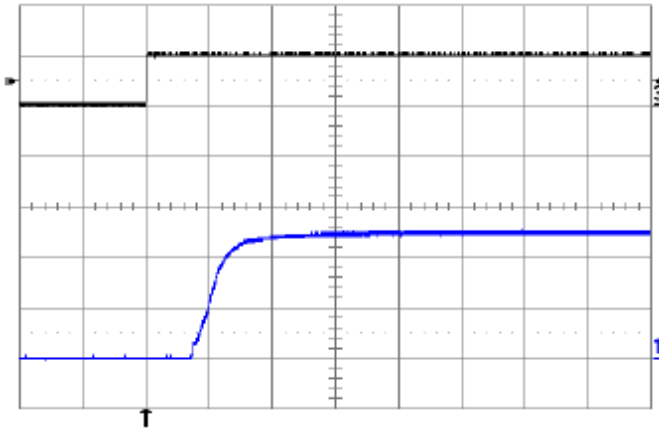
Fig. 5.0V.9: Turn-on transient at full rated load current (resistive) with no output capacitor at V_{in} = 48V , triggered via ON/OFF pin. Top trace: ON/OFF signal (5 V/div.). Bottom trace: output voltage (2 V/div.). Time scale: 2ms/div.
