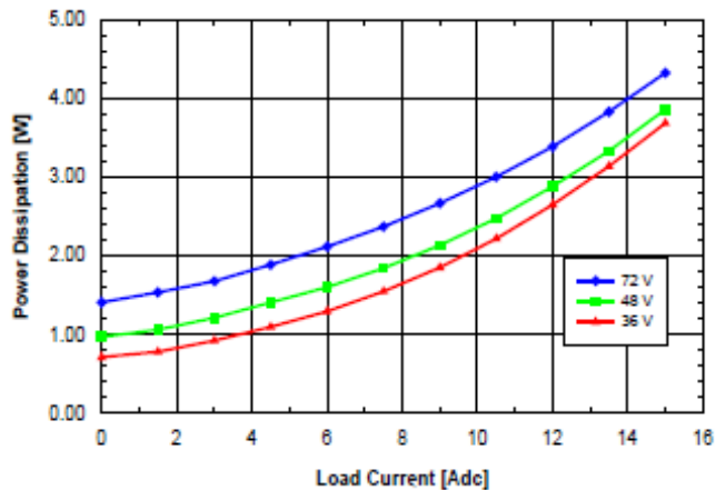
Fig. 1.2V.7: Power dissipation vs. load current and input voltage for SQ48T/S15012 converter mounted vertically with air flowing from pin 3 to pin 1 at a rate of 300 LFM (1.5 m/s) and T_a = 25^\circ\text{C} .
