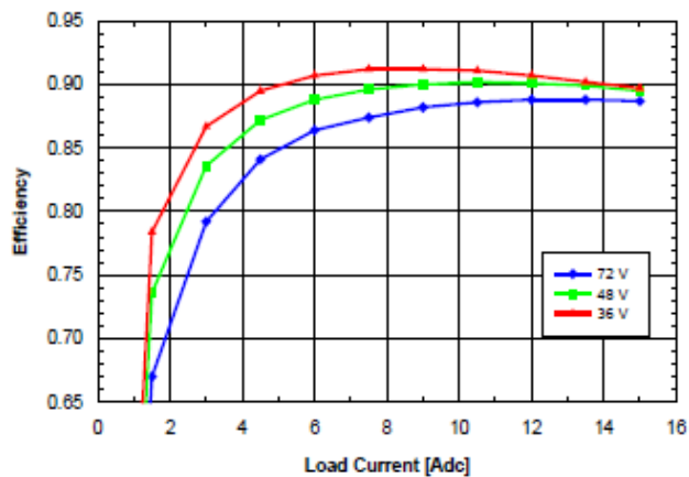
Fig. 3.3V.5: Efficiency vs. load current and input voltage for SQ48T/S15033 converter mounted vertically with air flowing from pin 3 to pin 1 at a rate of 300 LFM (1.5m/s) and T_a = 25^\circ\text{C} .
