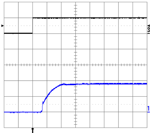
Fig. 1.8V.10: Turn-on transient at full rated load current (resistive) plus 10,000 \mu\text{F} at V_{in} = 48\text{ V} , triggered via ON/OFF pin. Top trace: ON/OFF signal (5 V/div.). Bottom trace: output voltage (1 V/div.). Time scale: 2 ms/div.
