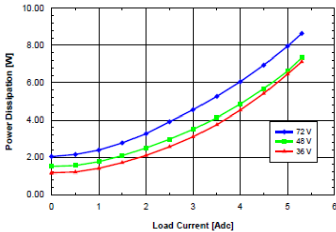
Fig. 8.0V.7: Power dissipation vs. load current and input voltage for SQ48T/S05080 converter mounted vertically with air flowing from pin 3 to pin 1 at a rate of 300 LFM (1.5 m/s) and T_a = 25^\circ\text{C} .
