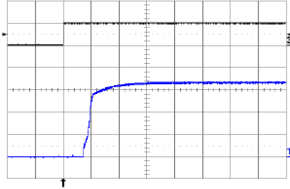
Fig. 3.3V.9: Turn-on transient at full rated load current (resistive) with no output capacitor at V_{in} = 48 V, triggered via ON/OFF pin. Top trace: ON/OFF signal (5 V/div.). Bottom trace: output voltage (1 V/div.). Time scale: 2 ms/div.
