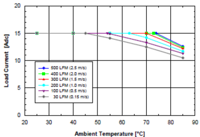
Fig. 3.3V.4: Available load current vs. ambient air temperature and airflow rates for SQ48S15033 converter mounted horizontally with Vin = 48V, air flowing from pin 3 to pin 1, and maximum FET temperature ≤ 120°C.
