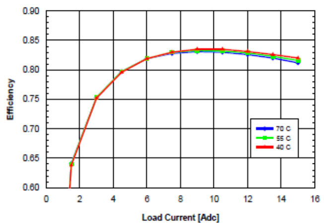
Fig. 1.2V.6: Efficiency vs. load current and ambient temperature for SQ48T/S15012 converter mounted vertically with V_{in} = 48 V and air flowing from pin 3 to pin 1 at a rate of 200 LFM (1.0 m/s).
