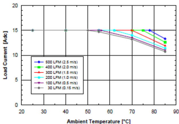
Fig. 3.3V.3: Available load current vs. ambient air temperature and airflow rates for SQ48S15033 converter mounted vertically with Vin = 48V, air flowing from pin 3 to pin 1, and maximum FET temperature ≤ 120°C.
