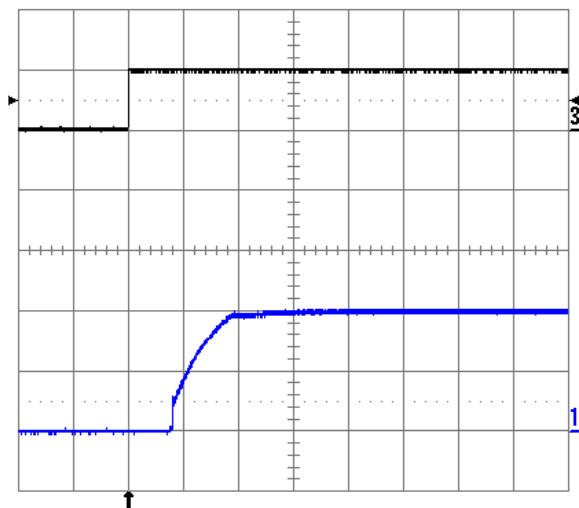
Fig. 2.0V.9: Turn-on transient at full rated load current (resistive) plus 10,000 \mu\text{F} at V_{in} = 48\text{ V} , triggered via ON/OFF pin. Top trace: ON/OFF signal (5 V/div.). Bottom trace: output voltage (1 V/div.). Time scale: 2 ms/div.
