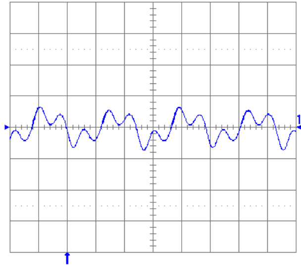
Fig. 2.5V.13: Output voltage ripple (20 mV/div.) at full rated load current into a resistive load with Co = 10 \mu F tantalum + 1 \mu F ceramic and Vin = 48 V. Time scale: 1 \mu s/div.
