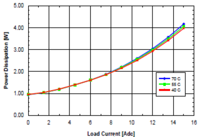
Fig. 1.0V.8: Power dissipation vs. load current and ambient temperature for SQ48T/S15010 converter mounted vertically with V_{in} = 48\text{ V} and air flowing from pin 3 to pin 1 at a rate of 200 LFM (1.0 m/s).
