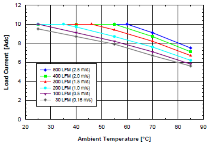
Fig. 5.0V.3: Available load current vs. ambient air temperature and airflow rates for SQ48S10050 converter mounted vertically with Vin = 48V, air flowing from pin 3 to pin 1, and maximum FET temperature ≤ 120°C.
