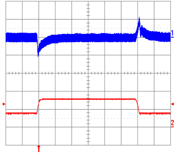
Fig. 2.5V.13: Output voltage ripple (20 mV/div.) at full rated load current into a resistive load with Co = 10 \mu F tantalum + 1 \mu F ceramic and Vin = 48 V. Time scale: 1 \mu s/div.
