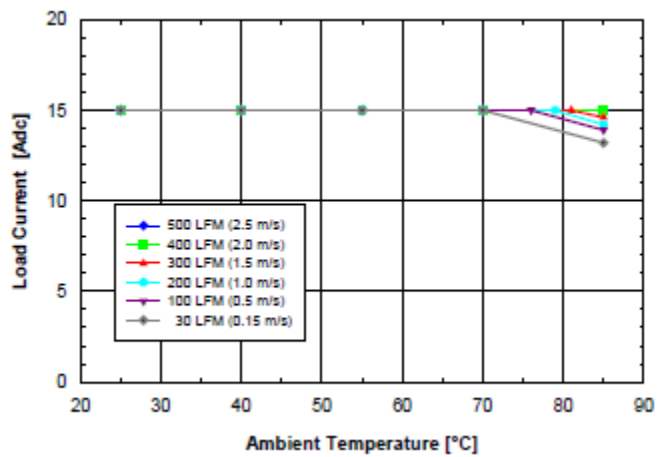
Fig. 1.8V.4: Available load current vs. ambient air temperature and airflow rates for SQ48S15018 converter mounted horizontally with V_{in} = 48 V, air flowing from pin 3 to pin 1, and maximum FET temperature \leq 120 °C.
