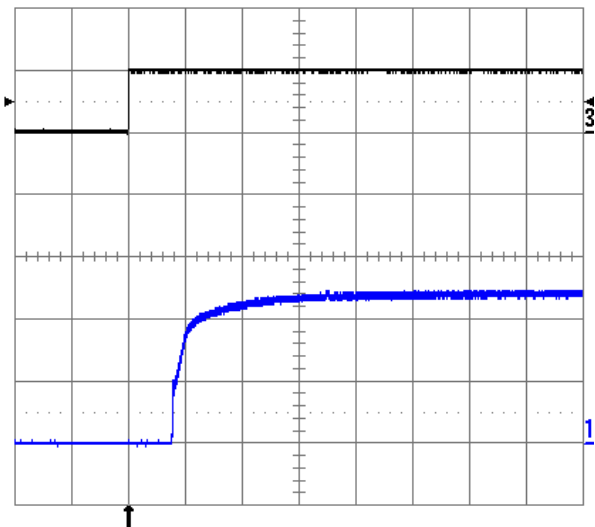
Fig. 1.2V.9: Turn-on transient at full rated load current (resistive) with no output capacitor at V_{in} = 48\text{ V} , triggered via ON/OFF pin. Top trace: ON/OFF signal (5 V/div.). Bottom trace: output voltage (0.5 V/div.). Time scale: 2 ms/div.
