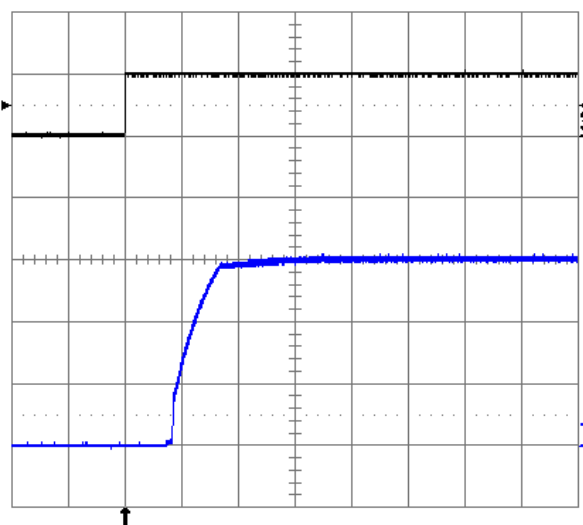
Fig. 1.5V.10: Turn-on transient at full rated load current (resistive) plus 10,000 \mu\text{F} at V_{in} = 48\text{ V} , triggered via ON/OFF pin. Top trace: ON/OFF signal (5 V/div.). Bottom trace: output voltage (0.5 V/div.). Time scale: 2 ms/div.
