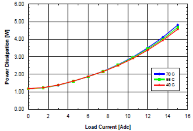
Fig. 1.8V.8: Power dissipation vs. load current and ambient temperature for SQ48T/S15018 converter mounted vertically with air flowing from pin 3 to pin 1 at a rate of 200 LFM (1.0 m/s).
