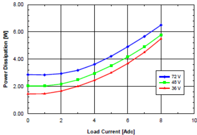
Fig. 6.0V.7: Power dissipation vs. load current and input voltage for SQ48T/S08060 converter mounted vertically with air flowing from pin 3 to pin 1 at a rate of 300 LFM (1.5 m/s) and T_a = 25^\circ\text{C} .
