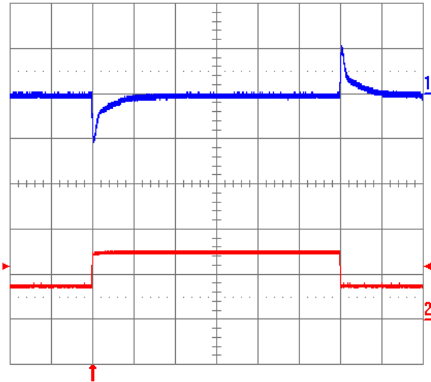
Fig. 1.8V.12: Output voltage response to load current step-change (3.75 A – 7.5 A – 3.75 A) at V_{in} = 48 V. Top trace: output voltage (100 mV/div.). Bottom trace: load current (5 A/div.). Current slew rate: 5 A/ \mu s. C_o = 450 \mu F tantalum + 1 \mu F ceramic. Time scale: 0.2 ms/div.
