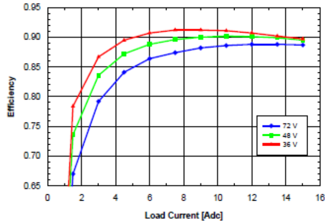
Fig. 2.5V.5: Efficiency vs. load current and input voltage for SQ48T/S15025 converter mounted vertically with air flowing from pin 3 to pin 1 at a rate of 300 LFM (1.5 m/s) and T_a = 25\text{ }^{\circ}\text{C} .
