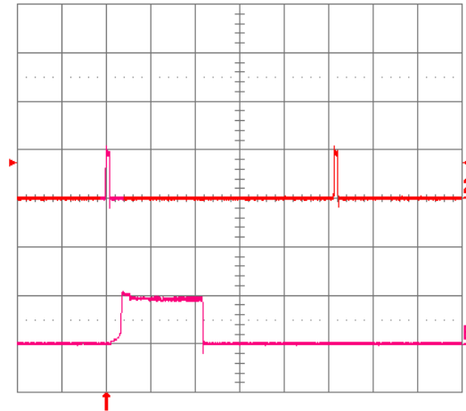
Fig. 3.3V.18: Load current (top trace, 20 A/div., 20 ms/div.) into a 10 mΩ short circuit during restart, at Vin = 48 V. Bottom trace (20 A/div., 1 ms/div.) is an expansion of the on-time portion of the top trace.
