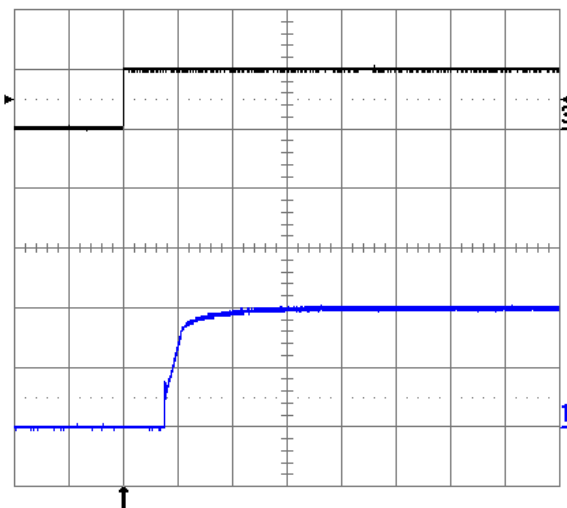
Fig. 2.0V.9: Turn-on transient at full rated load current (resistive) with no output capacitor at V_{in} = 48\text{ V} , triggered via ON/OFF pin. Top trace: ON/OFF signal (5 V/div.). Bottom trace: output voltage (1 V/div.). Time scale: 2 ms/div.
