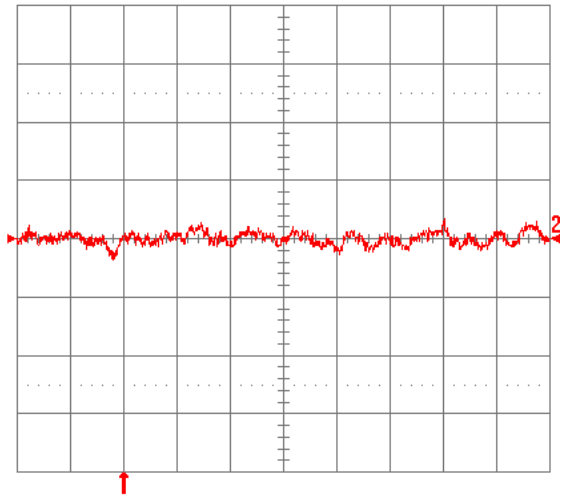
Fig. 1.5V.16: Input reflected ripple current, i_s (10 mA/div.), measured through 10 \mu H at the source at full rated load current and V_{in} = 48 V. Refer to Fig. 1.5V.14 for test setup. Time scale: 1 \mu s/div.
