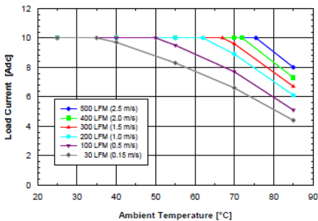
Fig. 5.0V.1: Available load current vs. ambient air temperature and airflow rates for SQ48T10050 converter with D height pins mounted vertically with Vin = 48V, air flowing from pin 3 to pin 1, and maximum FET temperature ≤ 120°C.
