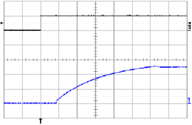
Fig. 5.0V.10: Turn-on transient at full rated load current (resistive) plus 10,000 \mu F at V_{in} = 48V , triggered via ON/OFF pin. Top trace: ON/OFF signal (5 V/div.). Bottom trace: output voltage (2 V/div.). Time scale: 2ms/div.
