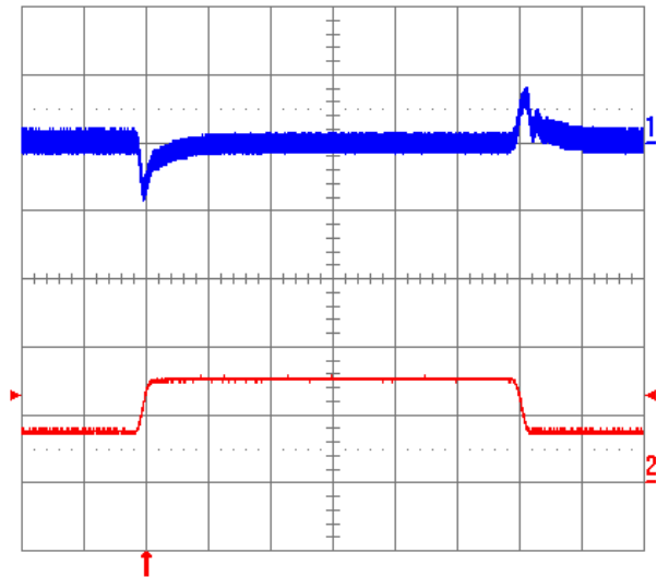
Fig. 1.5V.11: Output voltage response to load current step-change (3.75 A – 7.5 A – 3.75 A) at V_{in} = 48 V. Top trace: output voltage (100 mV/div.). Bottom trace: load current (5 A/div.). Current slew rate: 0.1 A/ \mu s. C_o = 1 \mu F ceramic. Time scale: 0.2 ms/div.
