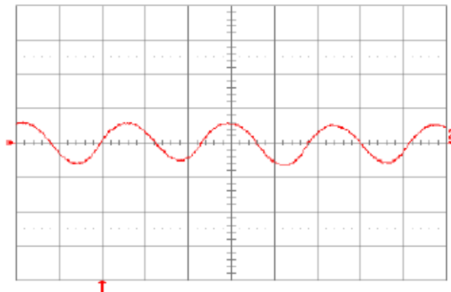
Fig. 5.0V.15: Input reflected ripple current, i_c (100 mA/div.), measured at input terminals at full rated load current and V_{in} = 48\text{V} . Refer to Fig. 5.0V.14 for test setup. Time scale: 1\ \mu\text{s}/\text{div} .
