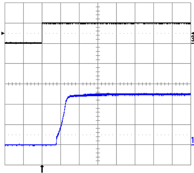
Fig. 2.5V.9: Turn-on transient at full rated load current (resistive) with no output capacitor at V_{in} = 48\text{V} , triggered via ON/OFF pin. Top trace: ON/OFF signal (5 V/div.). Bottom trace: output voltage (1 V/div.). Time scale: 2 ms/div.
