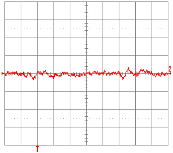
Fig. 1.2V.16: Input reflected ripple current, i_s (10 mA/div.), measured through 10 \mu H at the source at full rated load current and V_{in} = 48 V. Refer to Fig. 1.2V.14 for test setup. Time scale: 1 \mu s/div.
