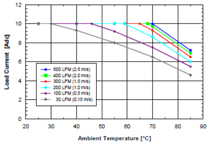
Fig. 5.0V.2: Available load current vs. ambient air temperature and airflow rates for SQ48T10050 converter with D height pins mounted horizontally with Vin = 48V, air flowing from pin 3 to pin 1, and maximum FET temperature ≤ 120°C.
