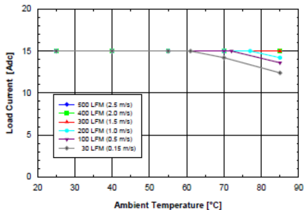
Fig. 2.OV.2: Available load current vs. ambient air temperature and airflow rates for SQ48T15020 converter with D height pins mounted horizontally with V_{in} = 48\text{ V} , air flowing from pin 3 to pin 1, and maximum FET temperature \leq 120^\circ\text{C} .
