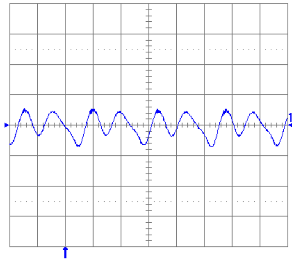
Fig. 1.2V.13: Output voltage ripple (20 mV/div.) at full rated load current into a resistive load with C_o = 10 \mu F tantalum + 1 \mu F ceramic and V_{in} = 48 V. Time scale: 1 \mu s/div.
