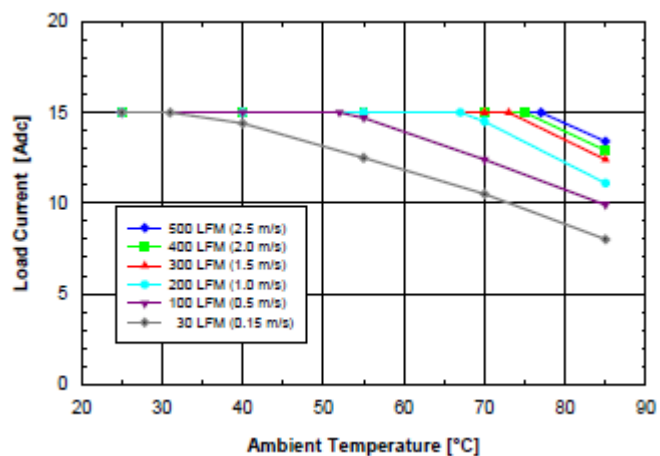
Fig. 3.3V.1: Available load current vs. ambient air temperature and airflow rates for SQ48T15033 converter with D height pins mounted horizontally with Vin = 48V, air flowing from pin 3 to pin 1, and maximum FET temperature ≤ 120°C.
