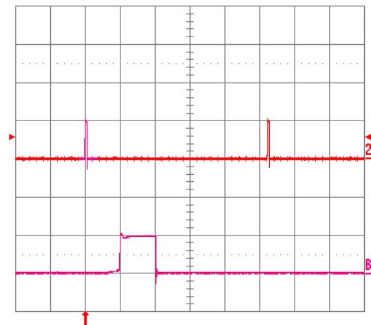
Fig. 1.5V.18: Load current (top trace, 20 A/div., 20 ms/div.) into a 10 m \Omega short circuit during restart, at V_{in} = 48 V. Bottom trace (20 A/div., 1 ms/div.) is an expansion of the on-time portion of the top trace.
