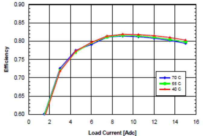
Fig. 1.0V.6: Efficiency vs. load current and ambient temperature for SQ48T/S15010 converter mounted vertically with V_{in} = 48\text{ V} and air flowing from pin 3 to pin 1 at a rate of 200 LFM (1.0 m/s).
