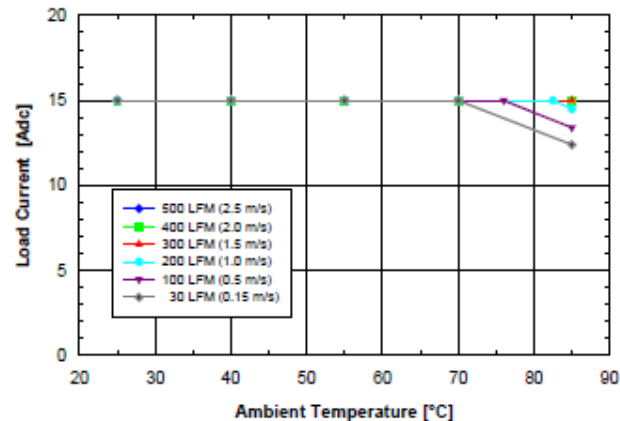
Fig. 1.5V.1: Available load current vs. ambient air temperature and airflow rates for SQ48T15015 converter with D height pins mounted vertically with V_{in} = 48\text{ V} , air flowing from pin 3 to pin 1, and maximum FET temperature \leq 120^\circ\text{C} .
