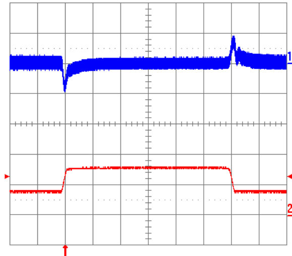
Fig. 1.2V.11: Output voltage response to load current step-change (3.75 A – 7.5 A – 3.75 A) at V_{in} = 48 V. Top trace: output voltage (100 mV/div.). Bottom trace: load current (5 A/div.). Current slew rate: 0.1 A/ \mu s. C_o = 1 \mu F ceramic. Time scale: 0.2 ms/div.
