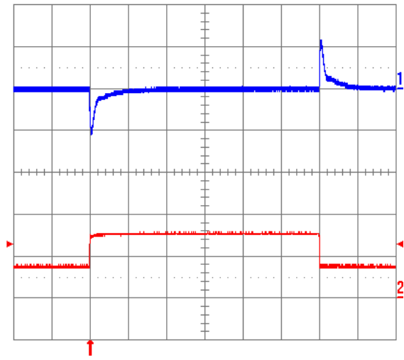
Fig. 1.2V.12: Output voltage response to load current step-change (3.75 A – 7.5 A – 3.75 A) at V_{in} = 48 V. Top trace: output voltage (100 mV/div.). Bottom trace: load current (5 A/div.). Current slew rate: 5 A/ \mu s. C_o = 450 \mu F tantalum + 1 \mu F ceramic. Time scale: 0.2 ms/div.
