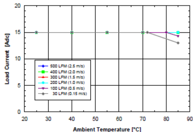
Fig. 1.2V.1: Available load current vs. ambient air temperature and airflow rates for SQ48T15012 converter with D height pins mounted vertically with V_{in} = 48\text{ V} , air flowing from pin 3 to pin 1, and maximum FET temperature \leq 120^\circ\text{C} .
