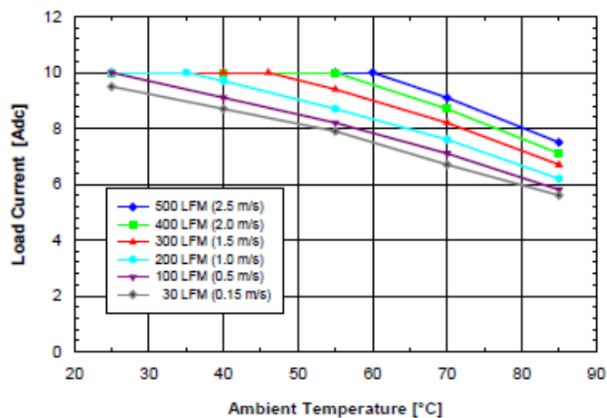
Fig. 5.0V.3: Available load current vs. ambient air temperature and airflow rates for SQ48S10050 converter mounted vertically with Vin = 48V, air flowing from pin 3 to pin 1, and maximum FET temperature ≤ 120°C.
