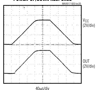
POWER-UP/DOWN RESPONSE
