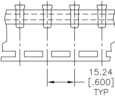
SPARE WIRE CAPS ON TAPE (SCALE 1:1)
