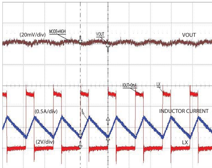
Steady State: MODE = High
