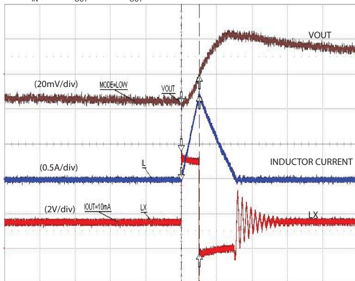
Steady State: MODE = Low
