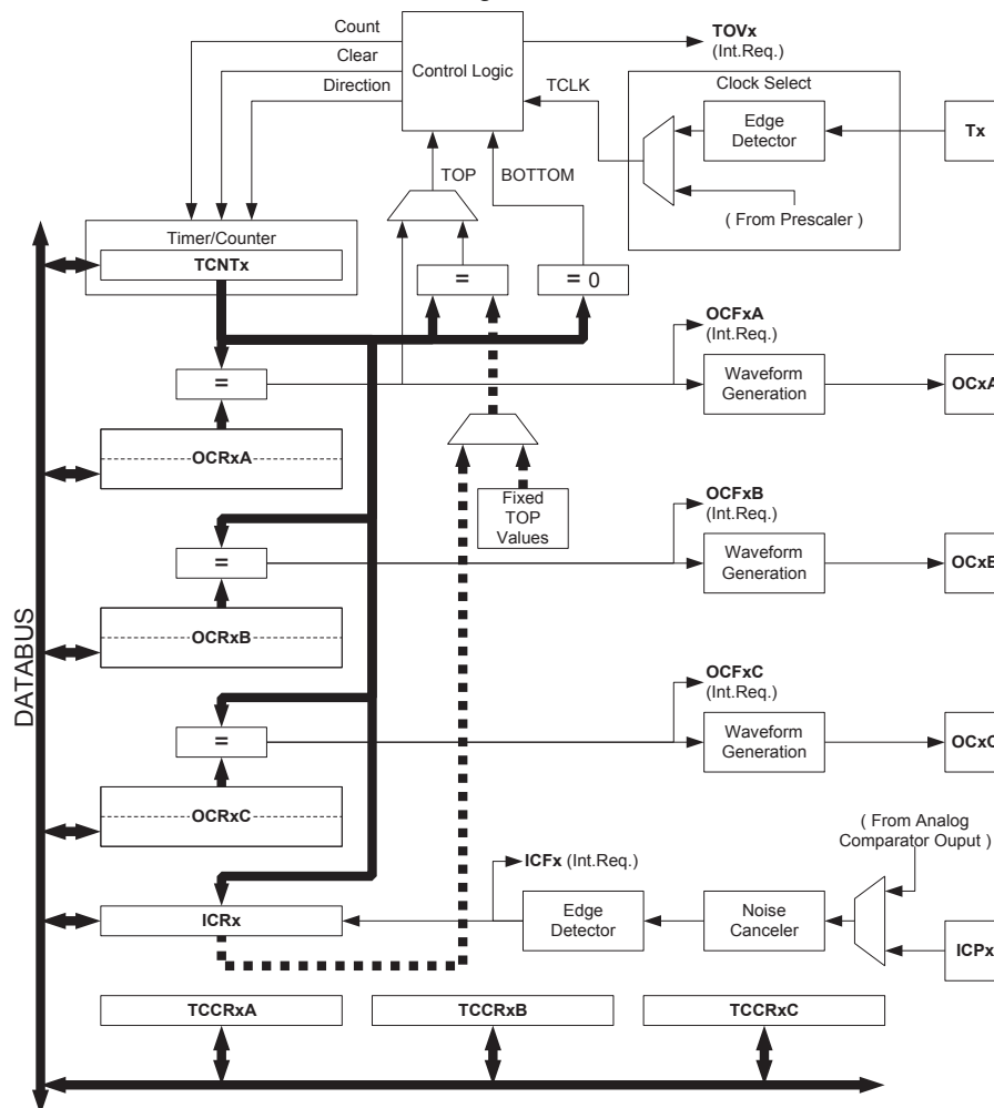
Figure 15-1. 16-bit Timer/Counter Block Diagram
