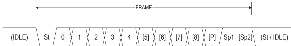
Figure 20-4. Frame Formats
