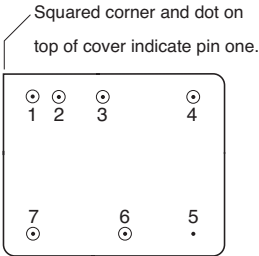
FIGURE 3: MCH PIN OUT
