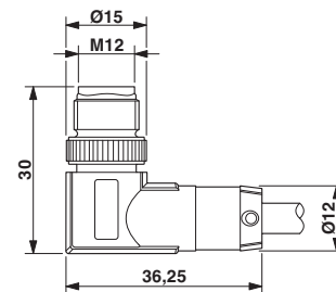
Dimensioned drawing
