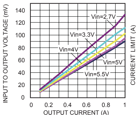
Input to Output Voltage vs. Load Current
