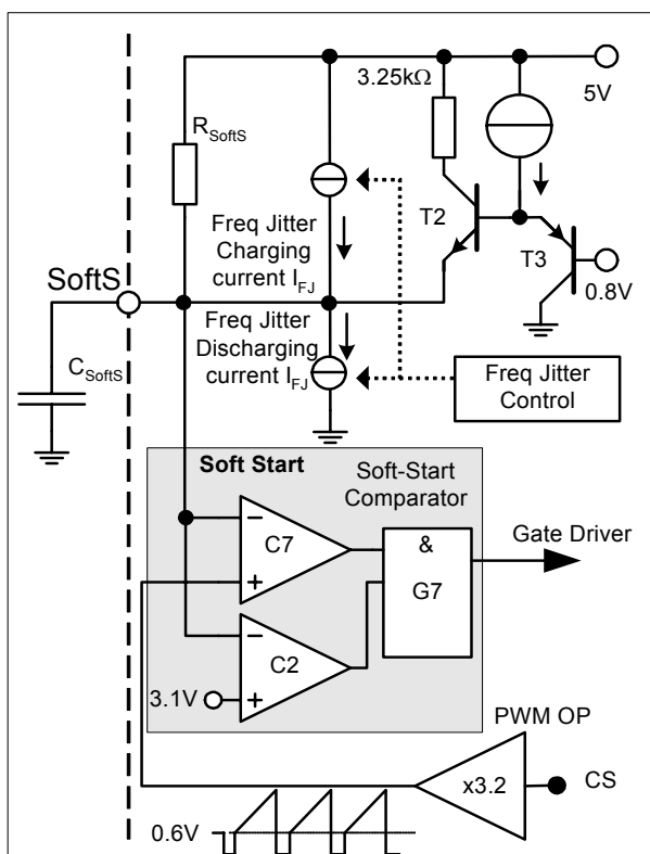
Figure 4 Soft Start
