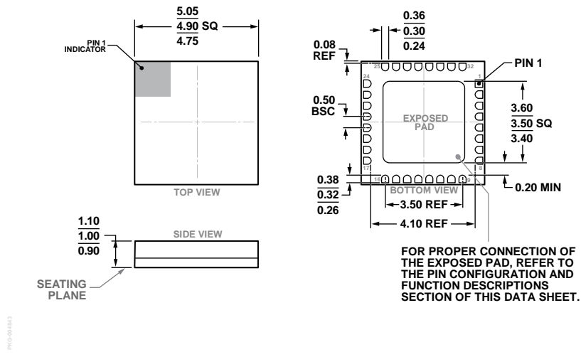
Figure 108. 32-Terminal Ceramic Leadless Chip Carrier [LCC] (E-32-1) Dimensions shown in millimeters
