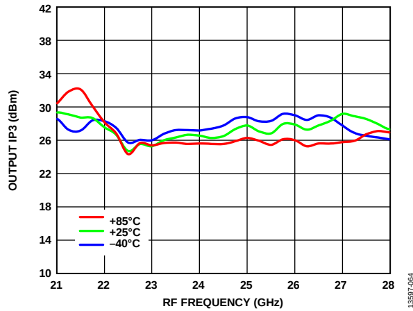
Figure 64. Output IP3 vs. RF Frequency over Temperature, LO Power = 4 dBm
