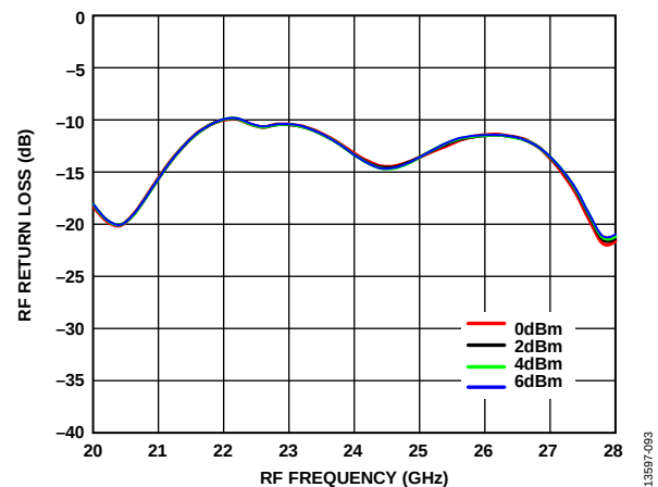
Figure 93. RF Return Loss vs. RF Frequency over LO Powers, LO Frequency = 12 GHz, T_A = 25^\circ\text{C}
