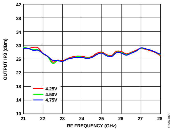
Figure 66. Output IP3 vs. RF Frequency over VDD1, LO Power = 4 dBm, T_A = 25^\circ\text{C}
