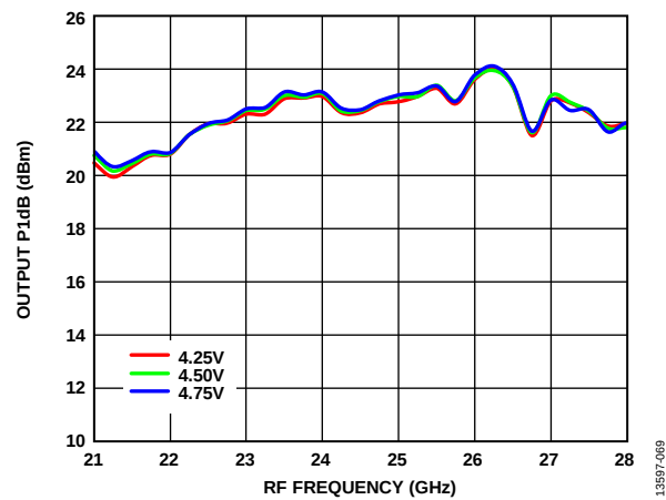
Figure 69. Output P1dB vs. RF Frequency over VDD1, LO Power = 4 dBm, T_A = 25^\circ\text{C}
