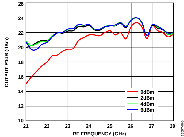
Figure 68. Output P1dB vs. RF Frequency over LO Powers, T_A = 25^\circ\text{C}
