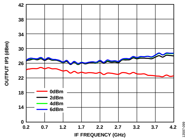
Figure 99. Output IP3 vs. IF Frequency over LO Powers, LO Frequency = 24 GHz, T_A = 25^\circ\text{C}
