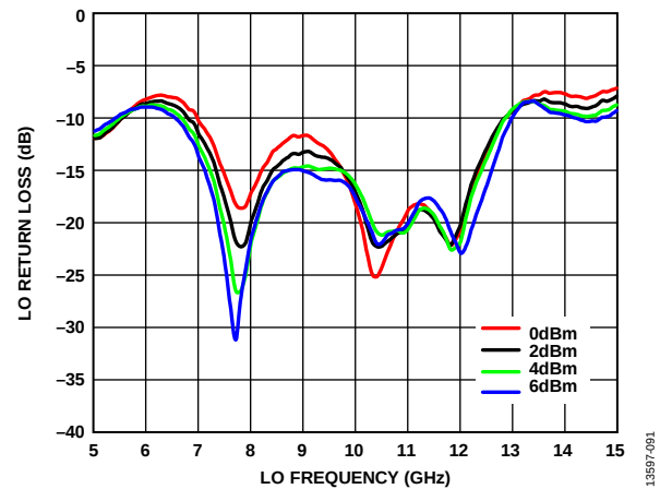
Figure 91. LO Return Loss vs. LO Frequency over LO Powers, T_A = 25^\circ\text{C}
