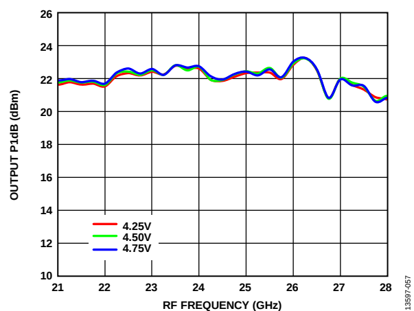
Figure 57. Output P1dB vs. RF Frequency over VDD1, LO Power = 4 dBm, T_A = 25^\circ\text{C}
