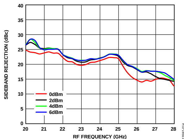
Figure 14. Sideband Rejection vs. RF Frequency over LO Powers, T_A = 25^\circ\text{C}
