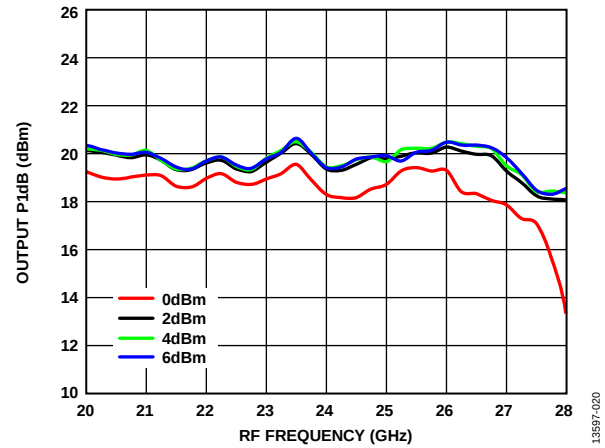
Figure 20. Output P1dB vs. RF Frequency over LO Powers, T_A = 25^\circ\text{C}
