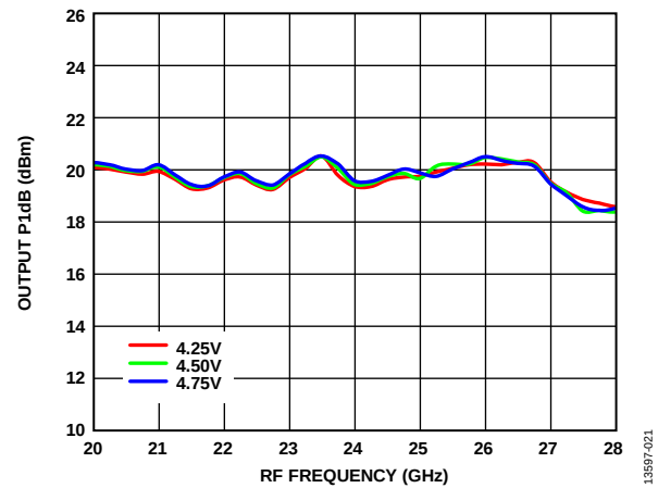
Figure 21. Output P1dB vs. RF Frequency over VDD1, T_A = 25^\circ\text{C}
