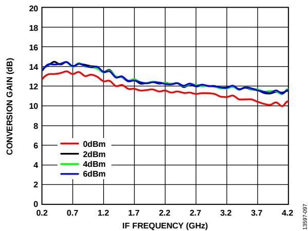
Figure 97. Conversion Gain vs. IF Frequency over LO Powers, LO Frequency = 12 GHz, T_A = 25^\circ\text{C}
