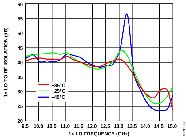
Figure 88. 1× LO to RF Isolation vs. 1× LO Frequency over Temperature, LO Power = 4 dBm
