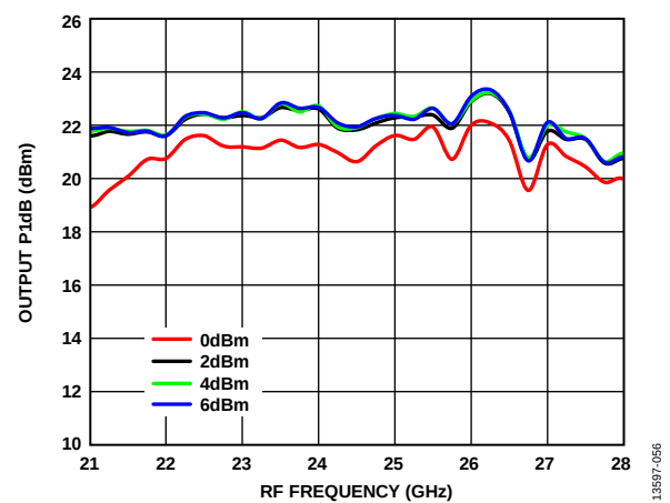
Figure 56. Output P1dB vs. RF Frequency over LO Powers, T_A = 25^\circ\text{C}
