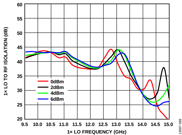
Figure 89. 1× LO to RF Isolation vs. 1× LO Frequency over LO Powers, T_A = 25^\circ\text{C}
