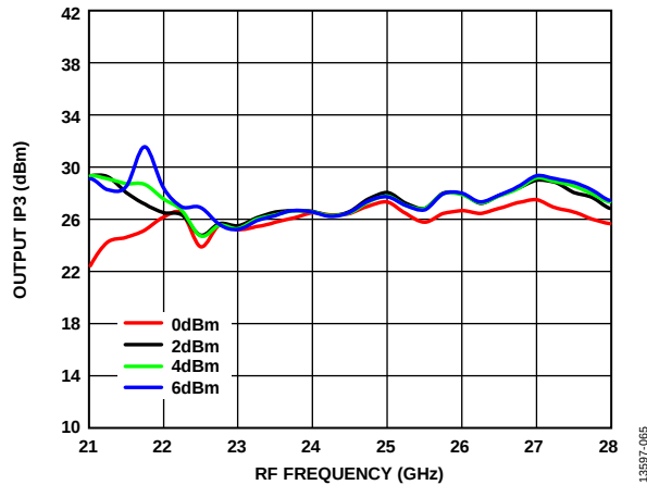
Figure 65. Output IP3 vs. RF Frequency over LO Powers, T_A = 25^\circ\text{C}
