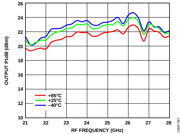
Figure 67. Output P1dB vs. RF Frequency over Temperature, LO Power = 4 dBm
