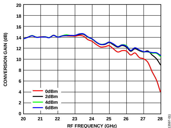
Figure 11. Conversion Gain vs. RF Frequency over LO Powers, T_A = 25^\circ\text{C}
