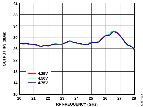
Figure 18. Output IP3 vs. RF Frequency over VDD1, T_A = 25^\circ\text{C}
