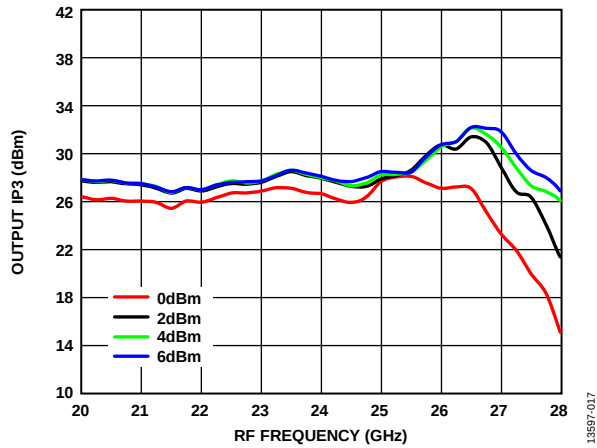
Figure 17. Output IP3 vs. RF Frequency over LO Powers, T_A = 25^\circ\text{C}
