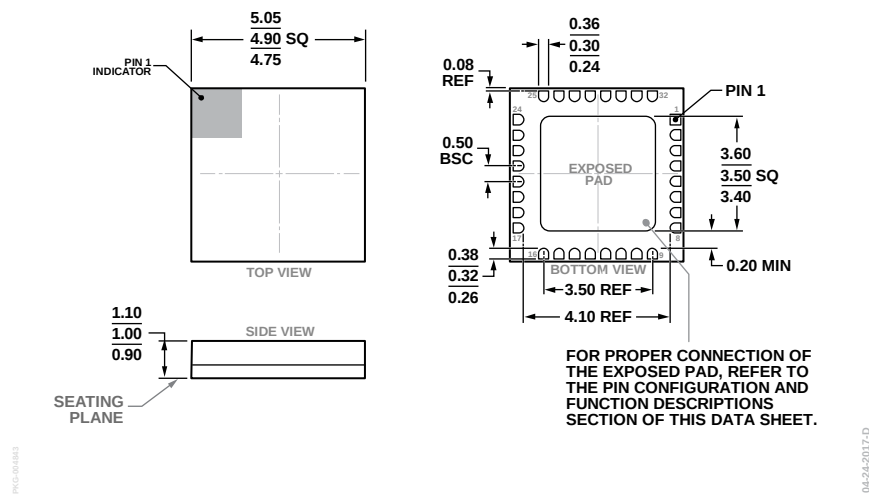
Figure 108. 32-Terminal Ceramic Leadless Chip Carrier [LCC] (E-32-1)
