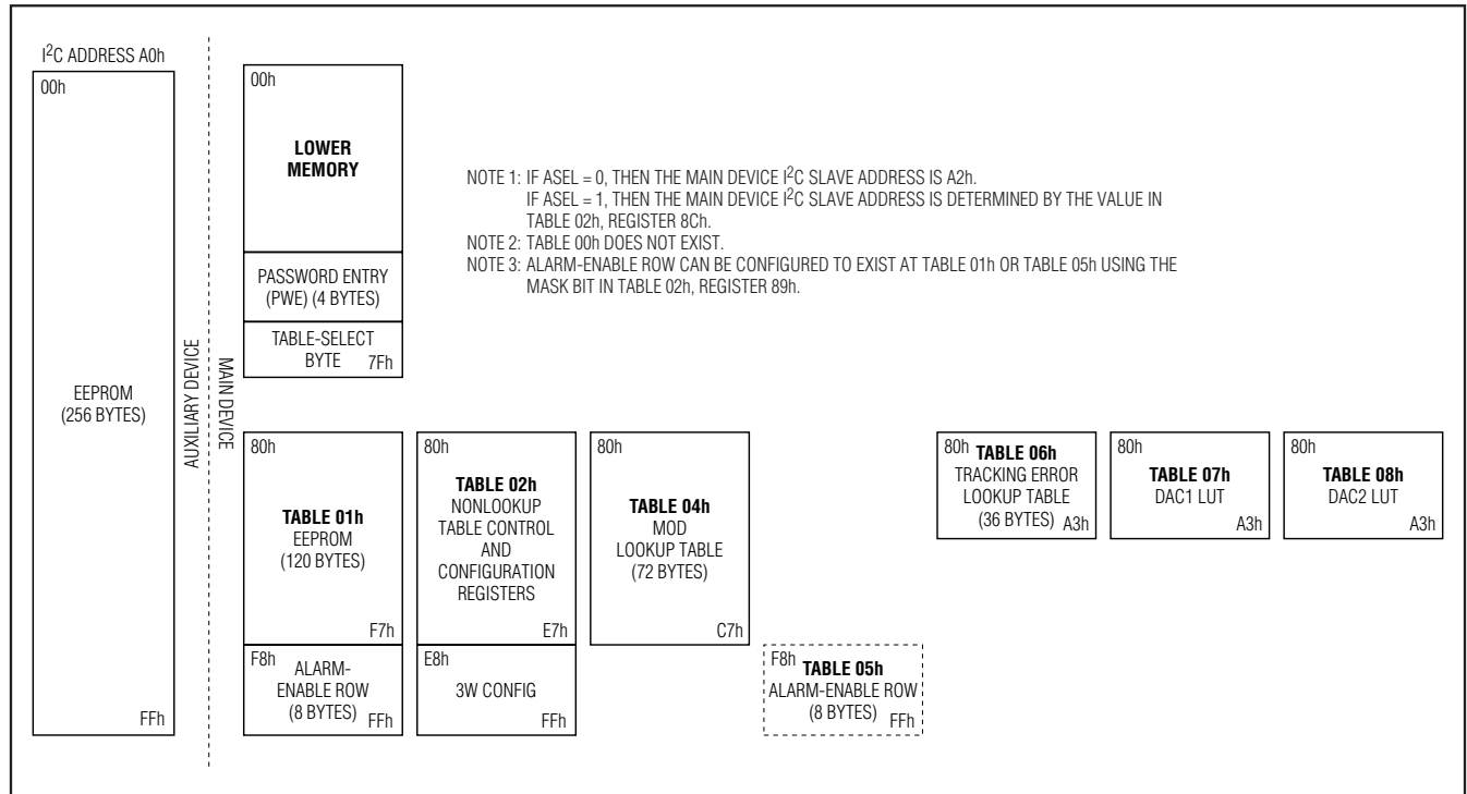
Figure 19. Memory Map
