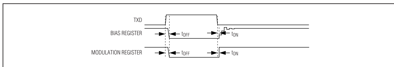
Figure 3. TXD Timing
