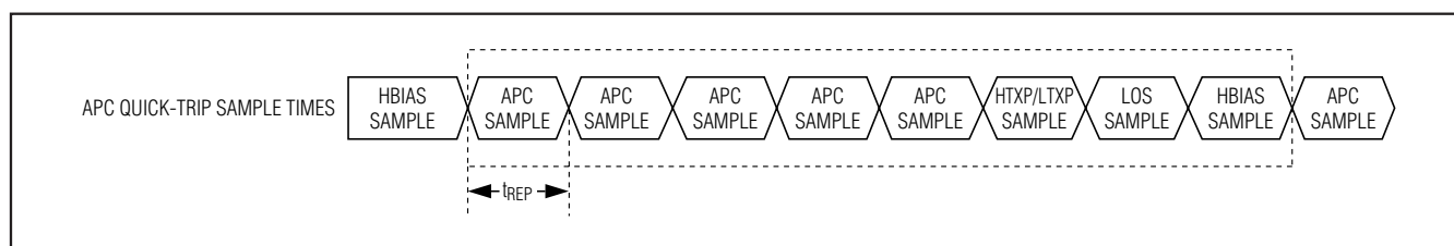
Figure 4. APC Loop and Quick-Trip Sample Timing
