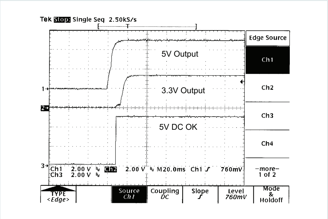
Figure 18 Start-up waveforms
