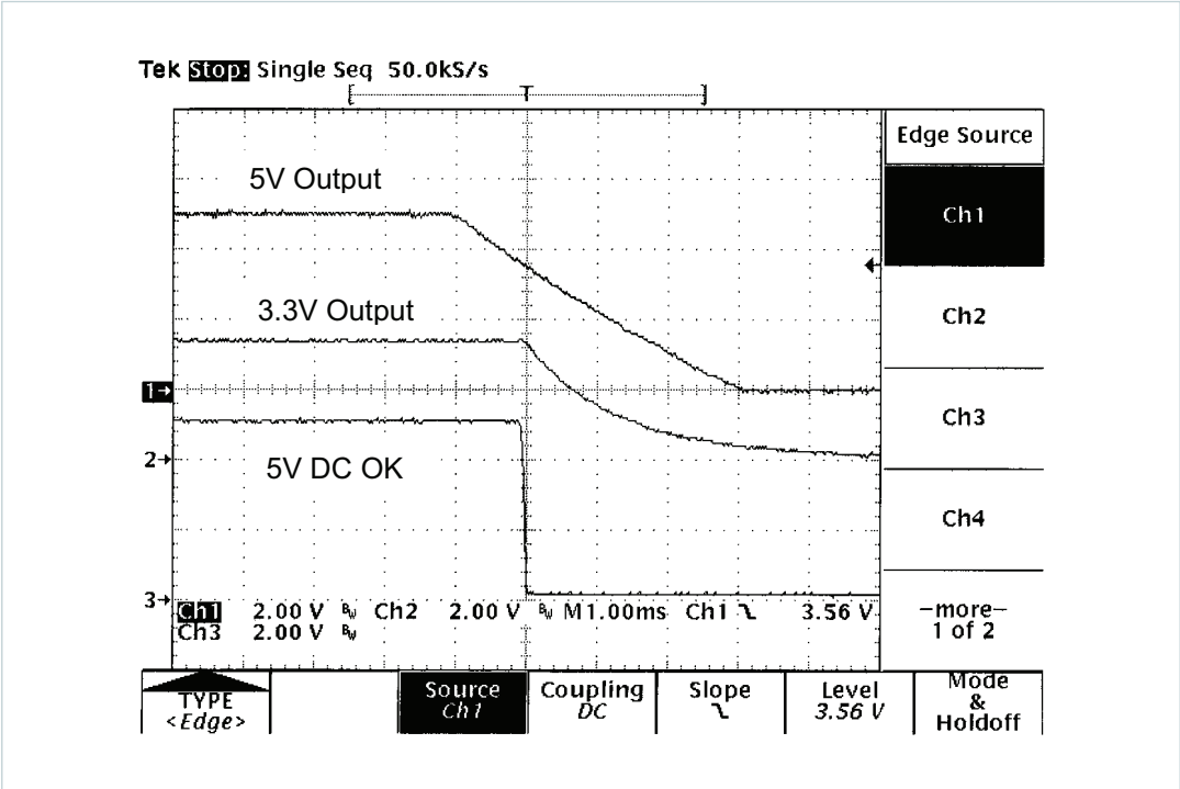
Figure 19 Shut-down waveforms
