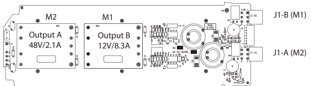
DUALQPAC - COMPONENT SIDE VIEW
