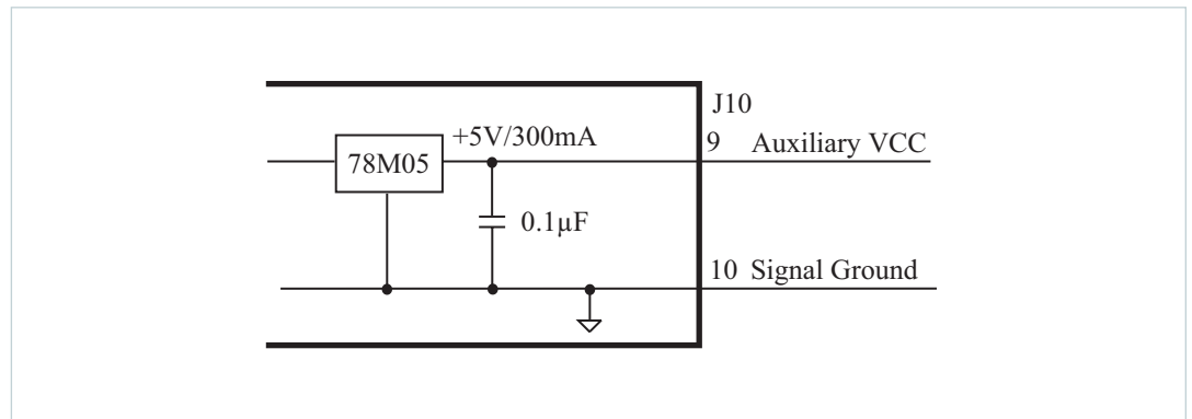
Figure 8 Auxiliary VCC
