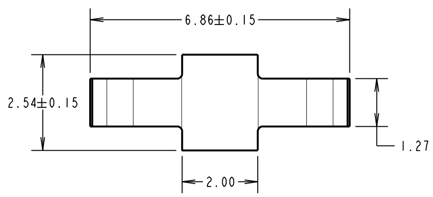
SINGLE COMPONENT DIMENSIONS
