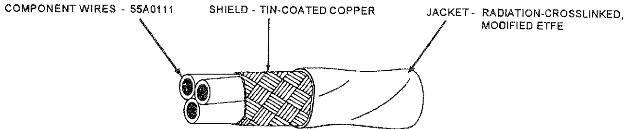
CABLE CONSTRUCTION DETAILS
