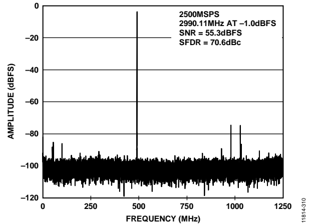
Figure 28. FFT Plot at 2.5 GSps, f_{IN} = 2990.11 MHz at AIN (SFDR = 70.6 dBc, SNR = 55.3 dBFS) (Input Network in Figure 75 Used)
