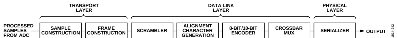
Figure 87. Data Flow
