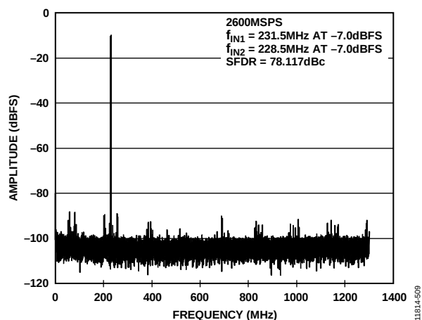
Figure 58. Two Tone FFT Plot at 2.6 GSPS AIN = 230 MHz
