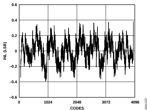
Figure 24. Integral Nonlinearity (INL), \pm 0.4\text{ LSB} at 2.0 GSPS
