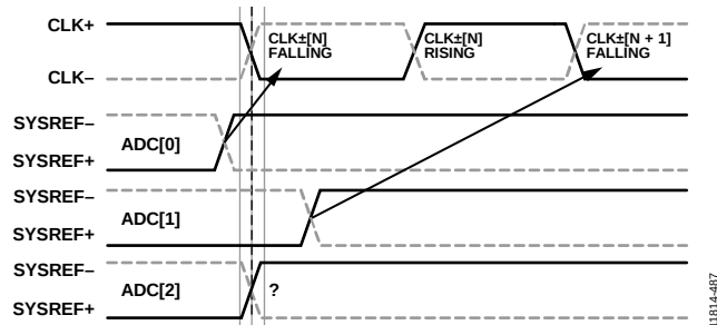
Figure 102. \text{SYSREF}_{\pm} Case From Three ADCs Having Various Phase Delays Relative to the Falling Edge of the Encode Clock and is Latched on Different Sample Clock Edges \text{CLK}_{\pm}[N] or \text{CLK}_{\pm}[N + 1]
