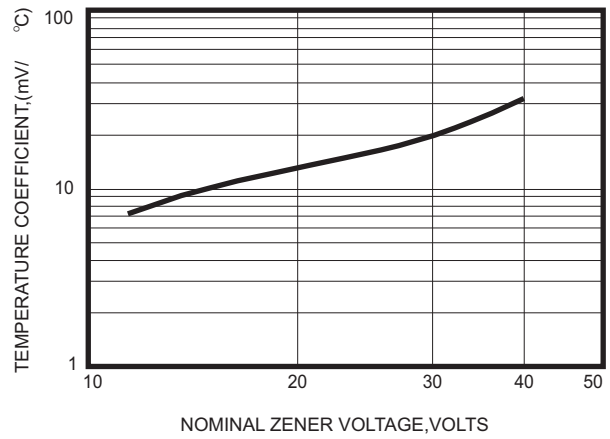
Fig.2 TEMPERATURE COEFFICIENTS
