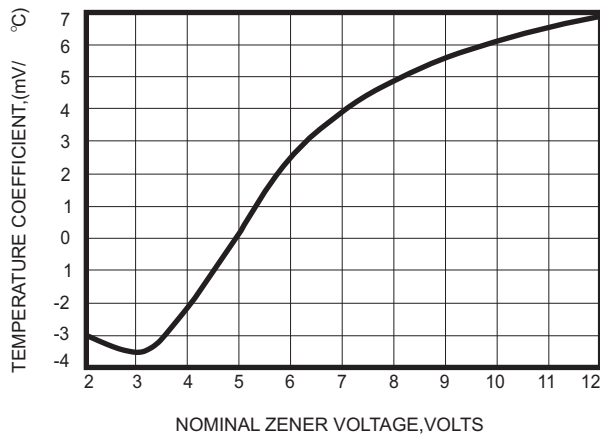
Fig.1 TEMPERATURE COEFFICIENTS
