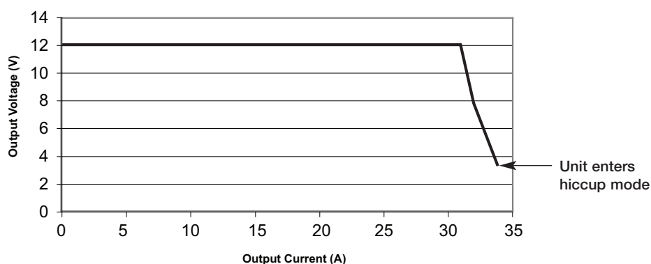
Figure 2 Typical V1 Overload Characteristic (MHP1000PS12 shown)
