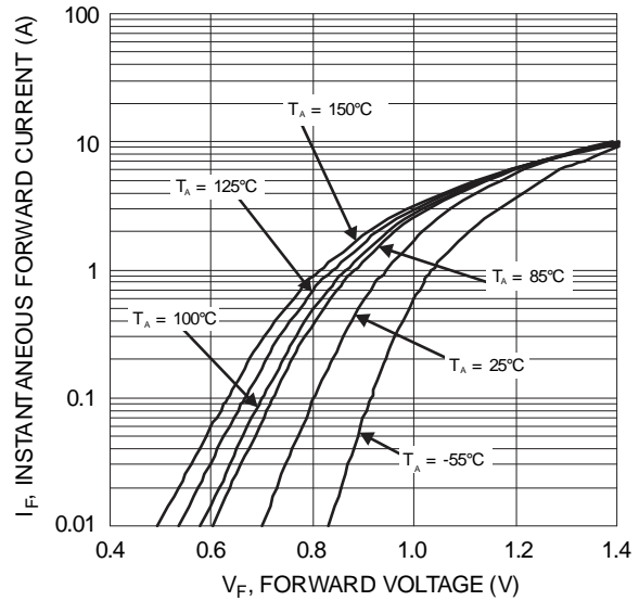
Figure 2 Instantaneous Forward Voltage
