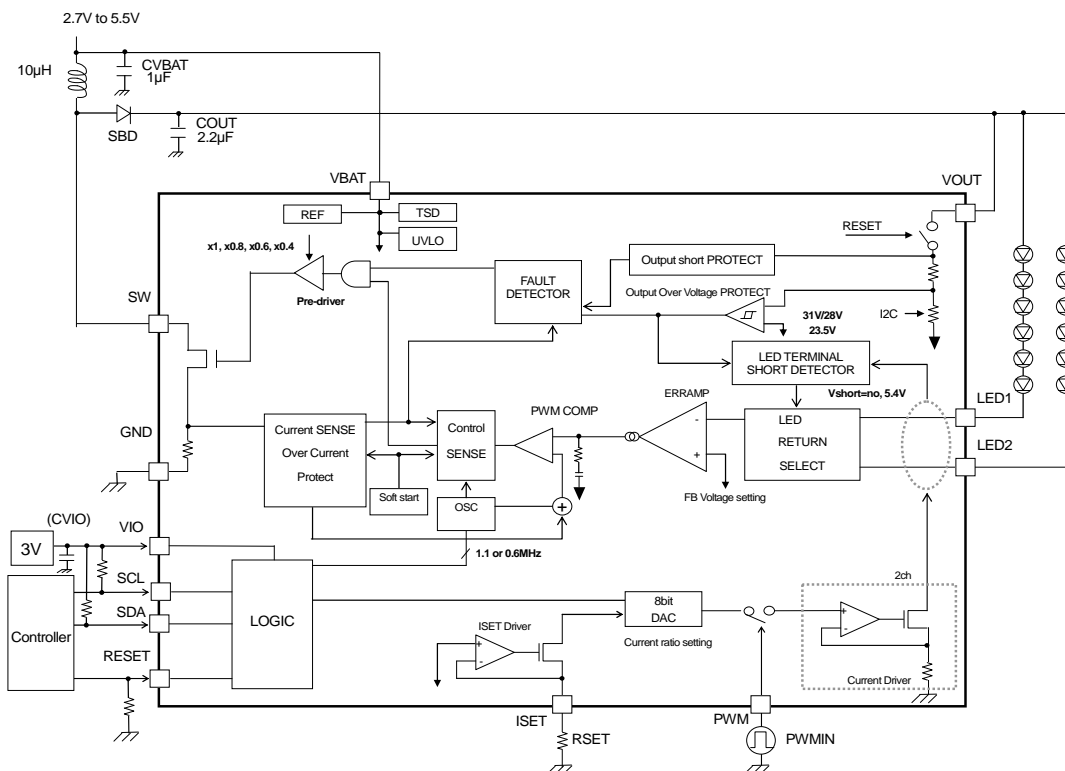
Figure 73. Schematic
