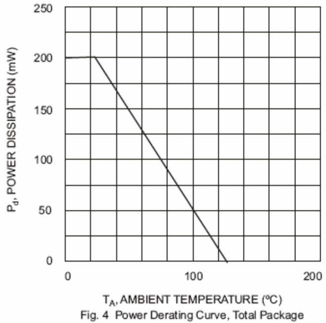
Fig. 4 Power Derating Curve, Total Package
