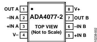
Figure 2. ADA4077-2 Pin Configuration, 8-Lead SOIC_N
