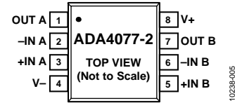
Figure 5. Pin Configuration, 8-Lead SOIC_N (R Suffix)
