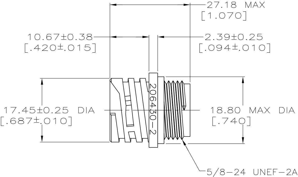
DETAIL B
