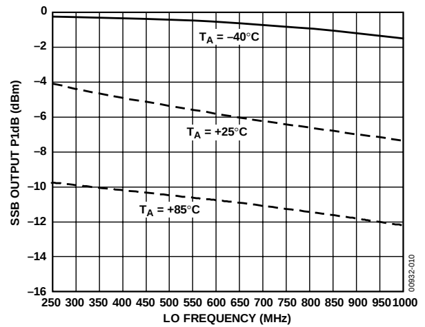
Figure 6. SSB Output 1 dB Compression Point ( OP1\text{dB} ) vs. F_{LO} ( V_S = 2.7\text{ V} , LO Level = -2\text{ dBm} , I and Q Inputs Driven in Quadrature, F_{BB} = 1\text{ MHz} )
