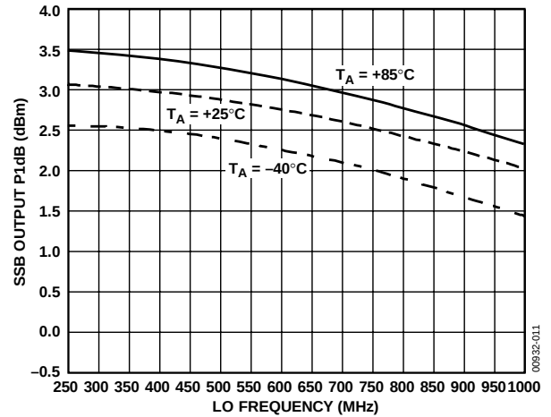
Figure 7. SSB Output 1 dB Compression Point ( OP1\text{dB} ) vs. F_{LO} ( V_S = 5\text{ V} , LO Level = -2\text{ dBm} , I and Q Inputs Driven in Quadrature, F_{BB} = 1\text{ MHz} )
