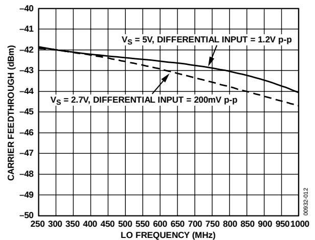
Figure 8. Carrier Feedthrough vs. F_{LO} (LO Level = -2\text{ dBm} , T_A = 25^\circ\text{C} )
