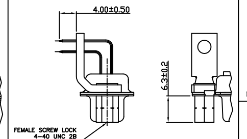
VIEW WITH RIVETED FEMALE SCREW &amp; METAL BRACKET
