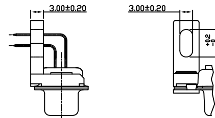
BRACKET DETAILS
