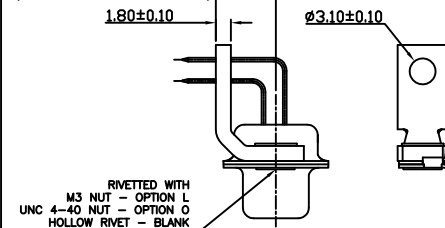
VIEW WITH RIVET &amp; METAL BRACKET
