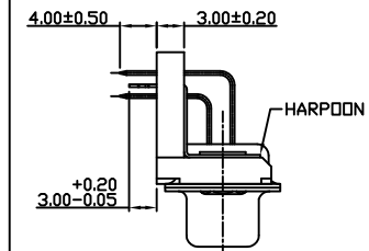
HARPOON WITH PLASTIC BRACKET
